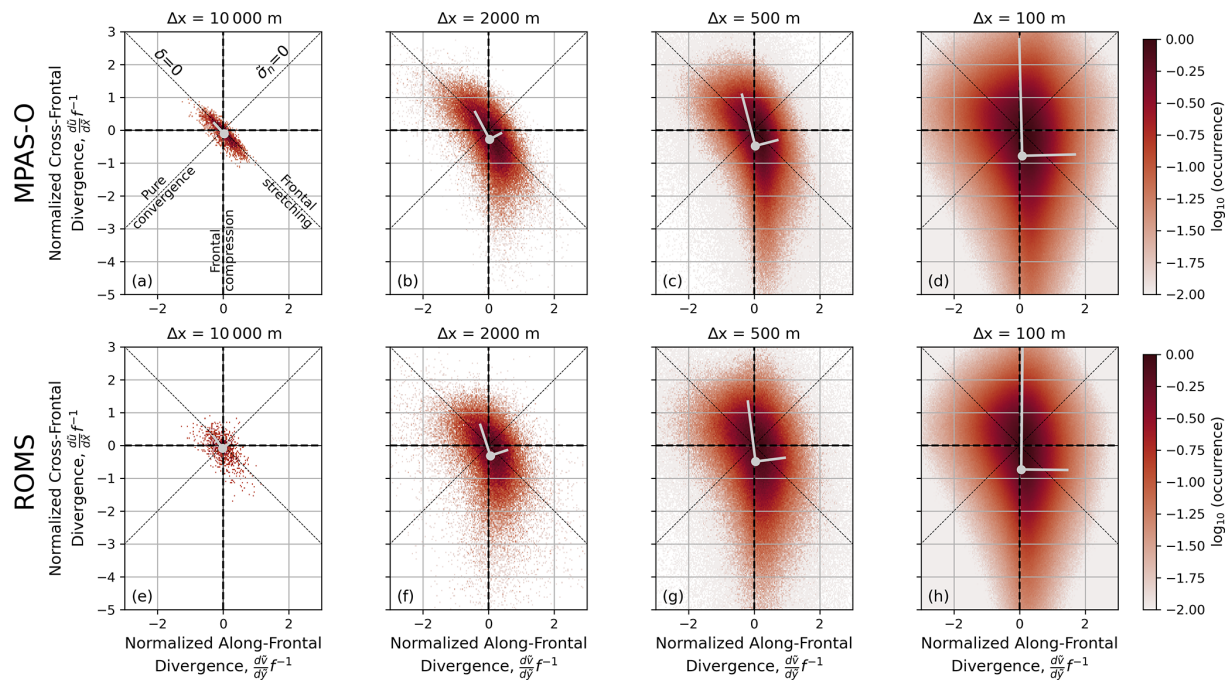
Figure 8. PDFs of normalized cross-frontal ( \frac{\partial \tilde{u}}{\partial \tilde{x}} f^{-1} ) vs. along-frontal ( \frac{\partial \tilde{v}}{\partial \tilde{y}} f^{-1} ) surface velocity gradients for MPAS-O (a–d) and ROMS (e–h) simulations over a range of spatial resolutions, for all points associated with frontal regions ( \zeta f^{-1} > 1 ). Colorbar denotes, in log scale, the frequency of occurrence of these relationships. Gray lines emanating from the average of these distributions (gray dots) show the principal components of variability of the distribution. The negatively sloping dashed line corresponds to zero divergence ( \delta = 0 ), while the positively sloping dashed line corresponds to zero effective strain ( \tilde{\sigma}_n = 0 ).
