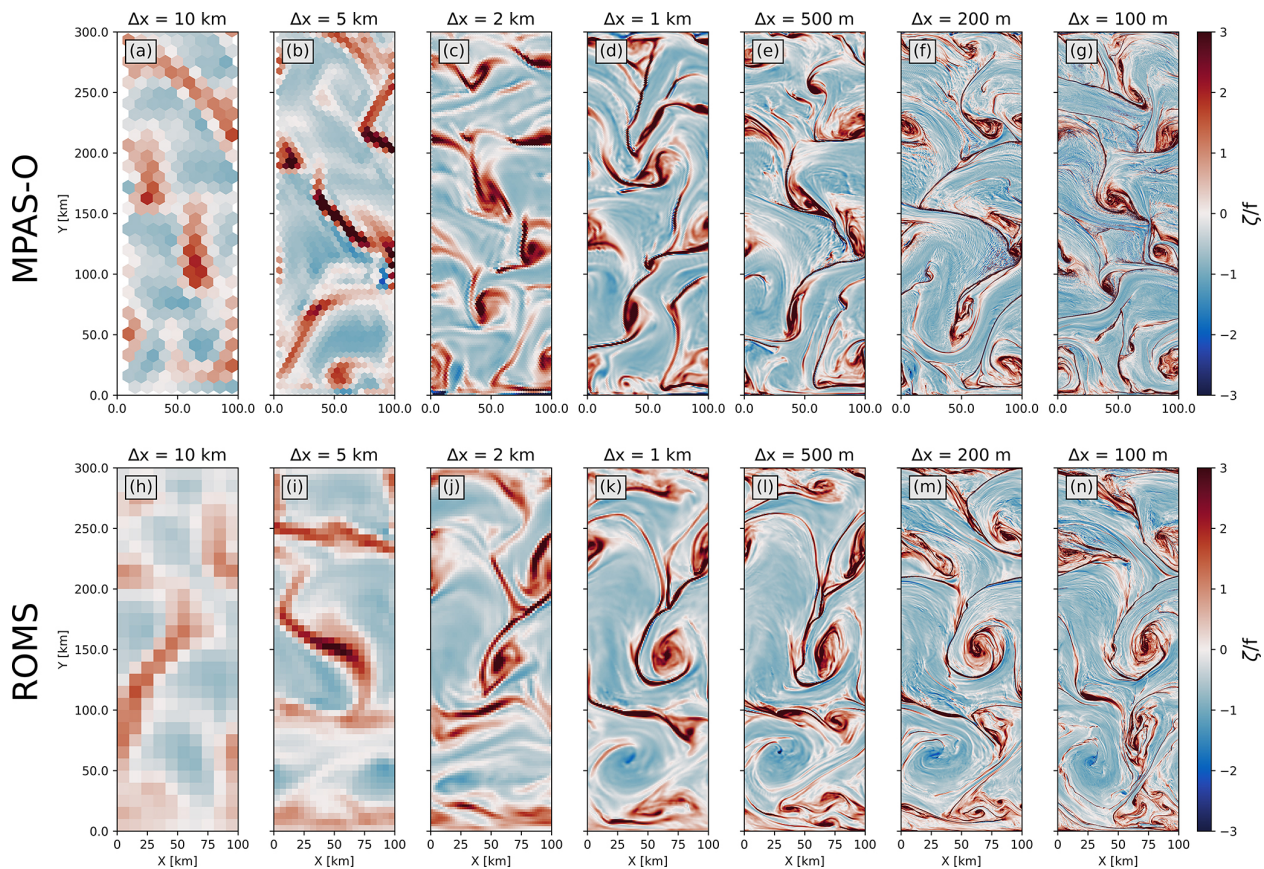
Figure 2. Snapshots of surface normalized relative vorticity ( \zeta f^{-1} ) plots for MPAS-O (a–g) and ROMS (h–n) on Day 12.
