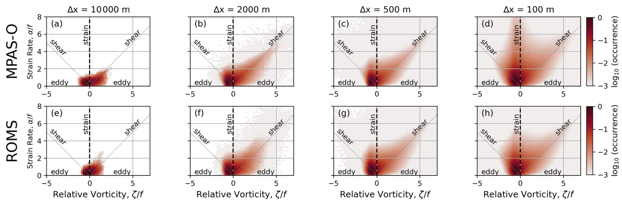
Figure 6. Joint PDFs of surface strain vs. surface relative vorticity for MPAS-O (a–d) and ROMS (e–h) simulations over a range of spatial resolutions. Colorbar denotes, in log scale, the frequency of occurrence of these relationships. Diagonal gray lines emanating at 45° to the left and right of the origin denote regions of shear while the vertical line identified at x = 0 corresponds to pure strain. Regions below these diagonal lines correspond to eddies in the simulations.
