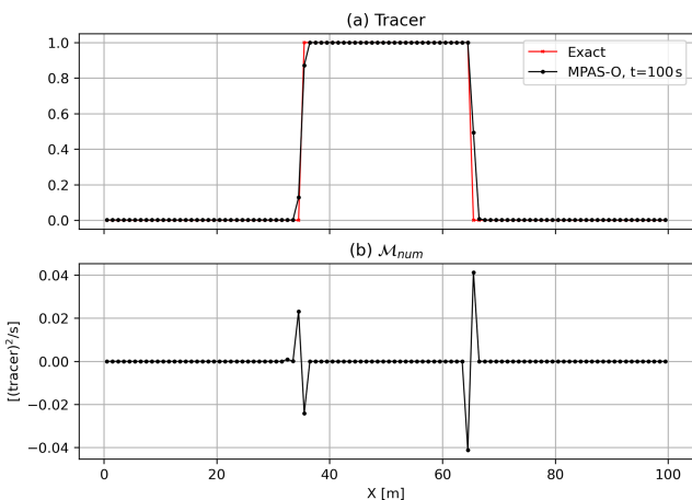
Figure B1. (a) Across-channel-averaged tracer and (b) numerical mixing at t = 100 s.
