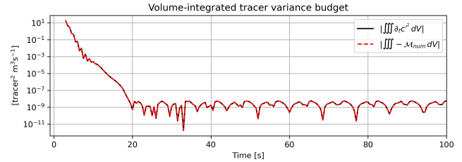
Figure B2. Volume-integrated tracer variance budget for the doubly periodic channel. The first several timesteps are omitted because |\mathcal{M}_{\text{num}}| is undefined at t = 0 and to account for the startup transient and two-step lag associated with the second-order Adams-Bashforth time-stepping scheme.
