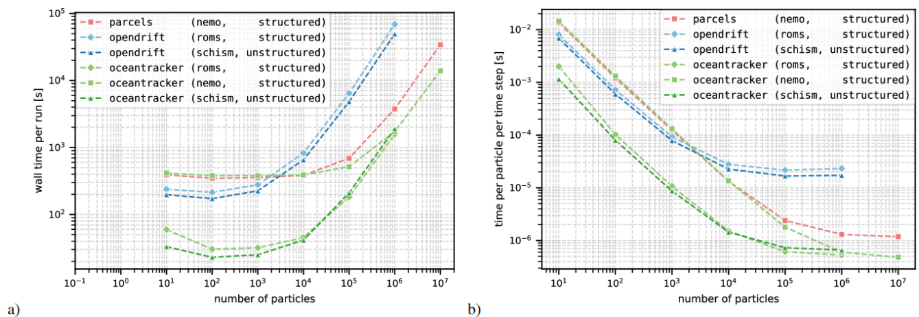
Figure 5. Computational comparison speed for OceanTracker with OpenDrift for structured (ROMS) and unstructured (SCHISM) grids, and with Parcels for structured (NEMO/GLORYS) grids. (a) Comparison of the total run time measured as wall time. (b) Normalized computational time per particle per RK4 time step.
