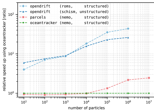
Figure 6. Comparison of the relative speed up from OceanTracker compared to OpenDrift and Parcels for the different data sets and particle sizes. The green line represents the baseline performance equal to OceanTracker.
