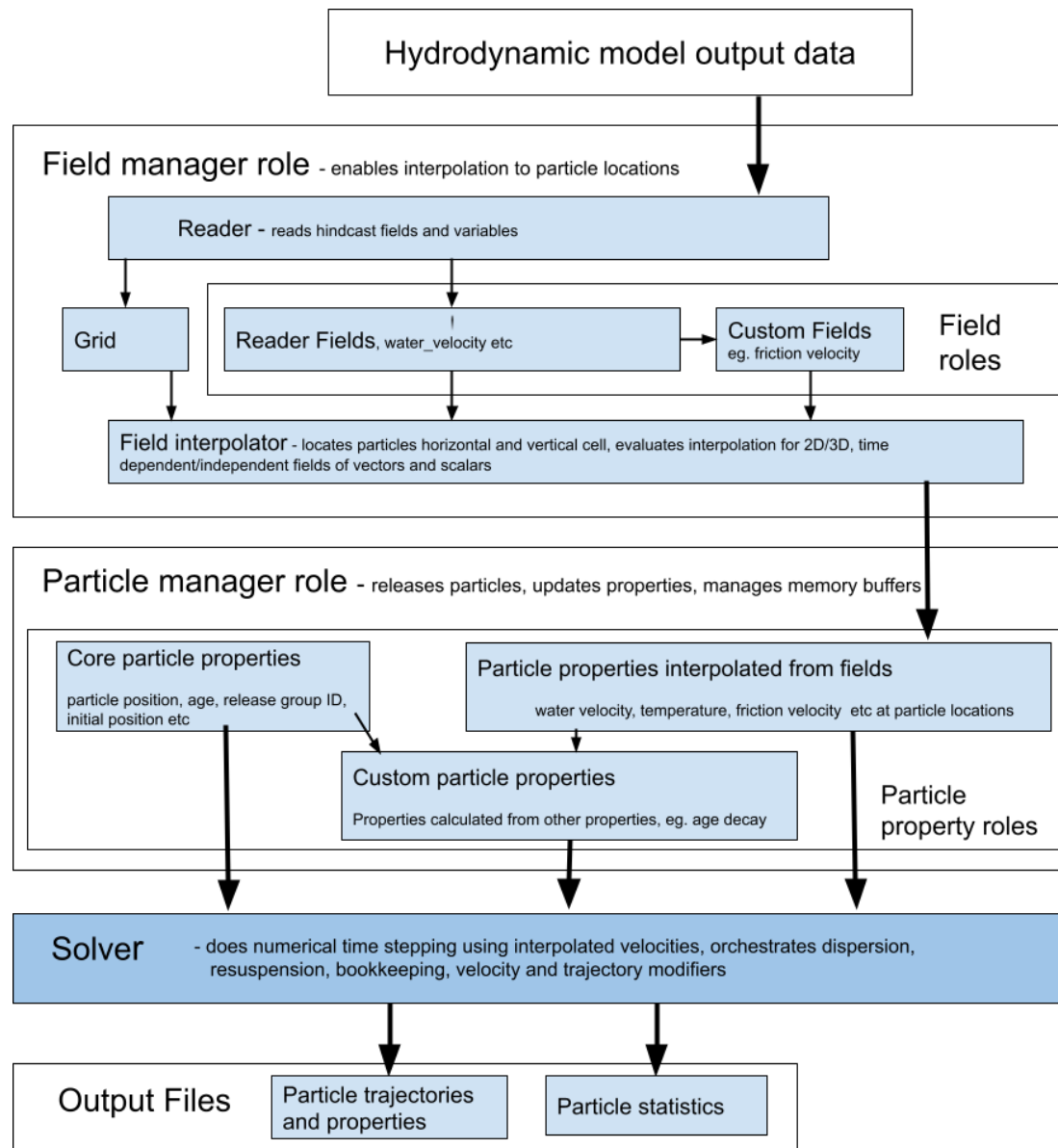
Figure 2. Outline of the data flow through the two main data structures, fields and particle properties, from hydrodynamic model files to output. These data structure roles are outlined in Sect. 4.2. Each has “managers” to orchestrate operations on the variants of each data structure, to deliver particle properties to the solver. The steps carried out by the solver are shown in Fig. 3.
