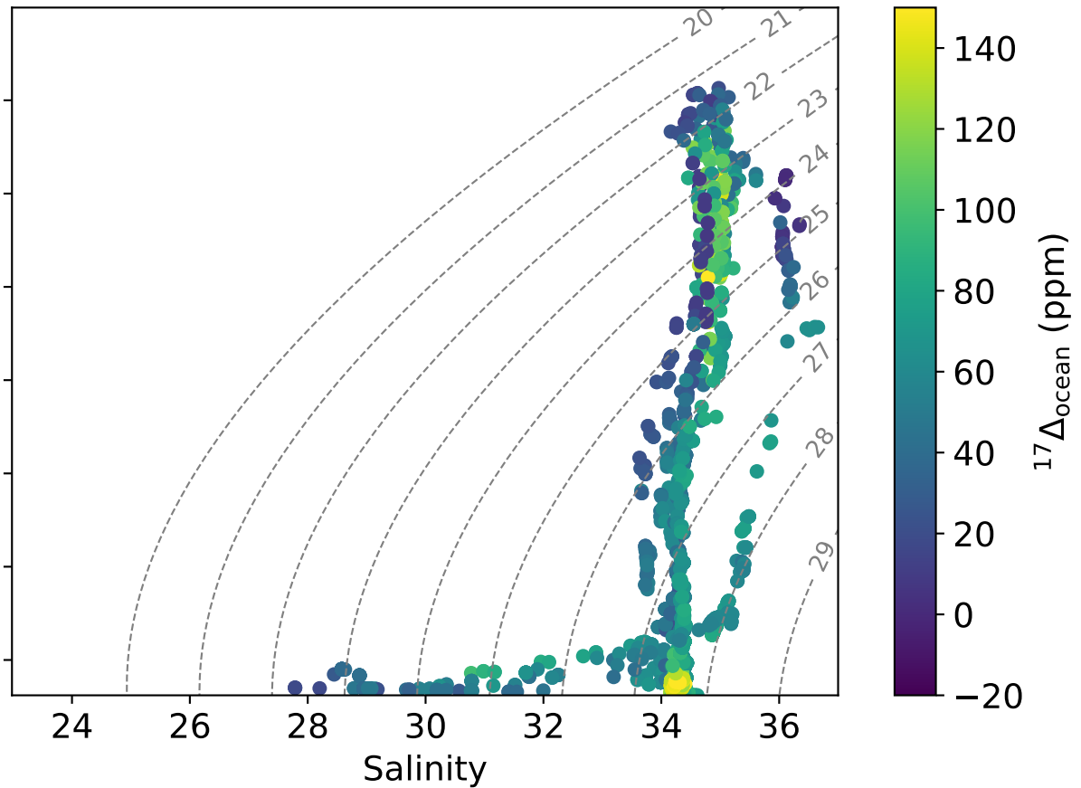
(b) CTRL simulation
