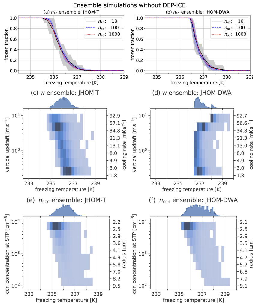
Figure 3. Ensemble simulations without DEP-ICE. Cumulative histograms of T_{\text{frz}} for the n_{\text{sd}} ensemble using (a) JHOM-T and (b) JHOM-DWA rates, respectively. Two-dimensional histograms of T_{\text{frz}} for the w ensemble using (c) JHOM-T and (d) JHOM-DWA rates, respectively. Two-dimensional histograms of T_{\text{frz}} for the n_{\text{ccn}} ensemble using (e) JHOM-T and (f) JHOM-DWA rates, respectively.
