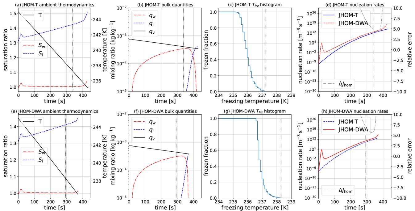
Figure 2. Air parcel ascent simulations for n_{sd} = 1000 using the JHOM-T (a–d) and JHOM-DWA (e–h) J_{hom} formulations, showing (a, e) ambient temperature T and saturation ratios with respect to water S_w and ice S_i , (b, f) bulk microphysical quantities, and (c, g) cumulative histograms of freezing temperatures T_{frz} . Panels (d) and (h) show the J_{hom} rates (solid lines indicate the active formulation, dashed lines the alternative formulation for comparison), as well as the relative difference between the JHOM-T and JHOM-DWA rates (grey). The vertical dashed line marks the first freezing event.
