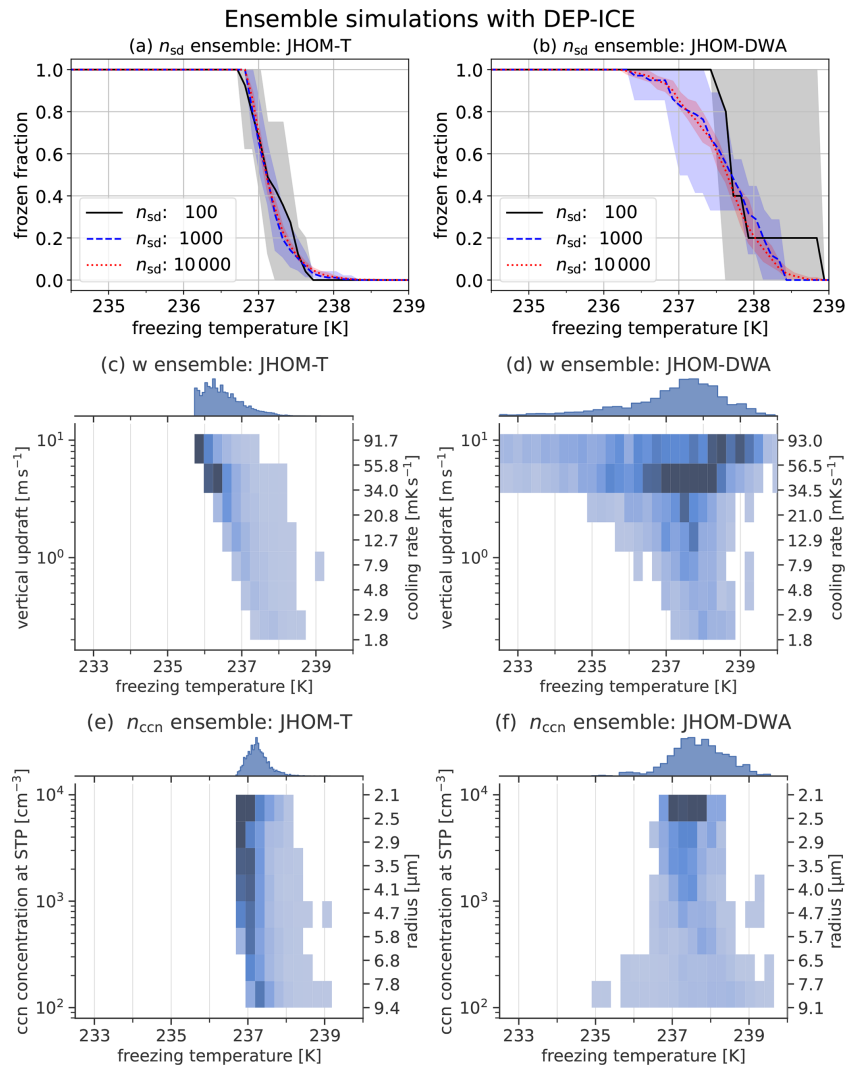
Figure 4. Ensemble simulations with vapour deposition on ice. Cumulative histograms of T_{frz} for the n_{sd} ensemble using (a) JHOM-T and (b) JHOM-DWA rates, respectively. Two-dimensional histograms of T_{frz} for the w ensemble using (c) JHOM-T and (d) JHOM-DWA rates, respectively. Two-dimensional histograms of T_{frz} for the n_{ccn} ensemble using (e) JHOM-T and (f) JHOM-DWA rates, respectively.
