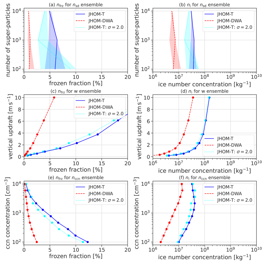
Figure 5. Frozen fraction n_{\text{frz}} for (a) the n_{\text{sd}} ensemble, (c) the w ensemble, (e) and the n_{\text{ccn}} ensemble. Ice number concentration n_i for (b) the n_{\text{sd}} ensemble, (d) the w ensemble, and (f) the n_{\text{ccn}} ensemble. Blue lines indicate simulations using the JHOM-T nucleation rate with monodisperse CCN spectra, teal lines the JHOM-T rate with lognormal CCN spectra, and red lines simulations using the JHOM-DWA rate. All simulations were performed with n_{\text{sd}} = 10000 and vapour deposition on ice active.
