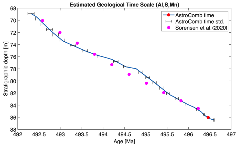
Figure 9. Timescale computed from the multi-channel data using the S, Al and Mn records. See Fig. 8 caption for further details.
