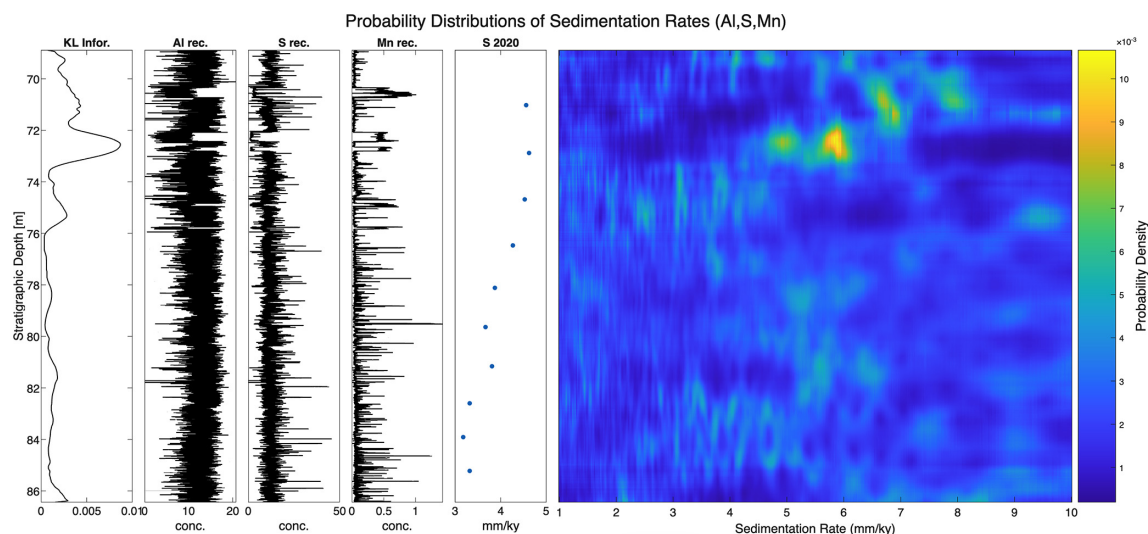
Figure 6. Probabilistic analysis of sedimentation rates in the Fågeltofta-2 core, based on simultaneous processing of S, Al, and Mn. Comparing to Fig. 5 it is clear that this multi-channel analysis has provided a higher resolution with more distinct peaks in the probability densities. Below 76 m, the information content is smaller where spectral peaks are few and/or less pronounced.
