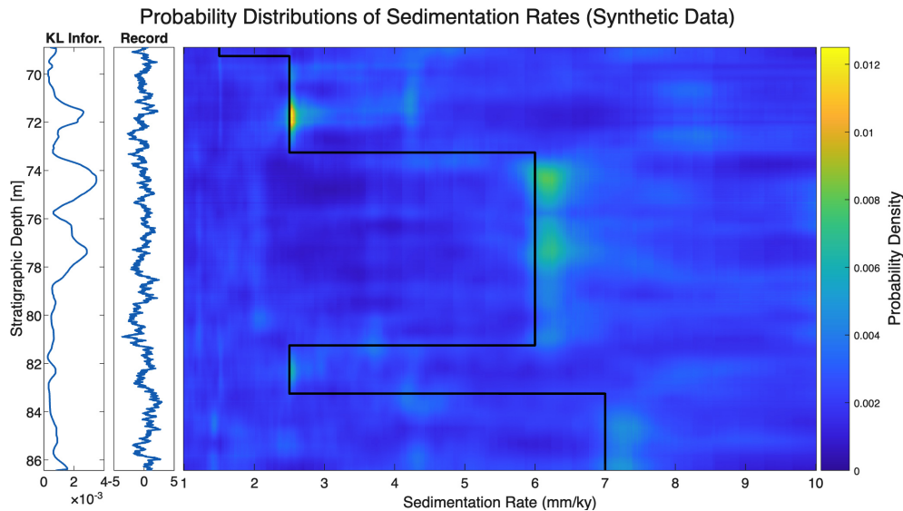
Figure 2. Probability density distributions of sedimentation rates computed from synthetic data with 200 % red noise (“Record” shown on the 2nd plot from left). The synthetic reference model is overlain (black curve) to illustrate the fidelity of the reconstruction. Visually, the reconstructed sedimentation rates closely reproduce the true reference model. However, the results also demonstrate that noise, together with ambiguity in assigning a given cycle to different target periods, can introduce artifacts and lead to multimodal sedimentation-rate probability distributions for a given depth. Information content (Kullback–Leibler information) is shown in the left plot. Lower information content below 79 m depth, albeit with local peaks near 82.3 and 86.1 m, reflect fewer and/or less pronounced peaks within the sliding window.
