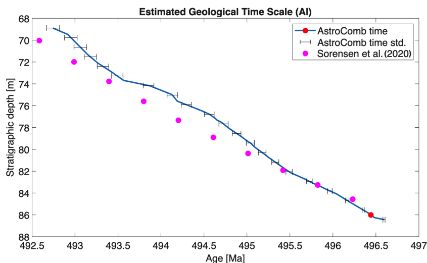
Figure 8. Estimated geological timescale and its uncertainty (standard deviation of a Gaussian approximation to the posterior near the computed time), based on probabilistic estimation of instantaneous sedimentation rates from the Al record in the Fågeltofta-2 core. Each time is a MAP estimate computed under the assumption of independency between neighbouring layers. The timescale is anchored at 86.005 m, corresponding to 496 595 kyr (Sørensen et al., 2020). This anchor is marked with a red circle on the graph.
