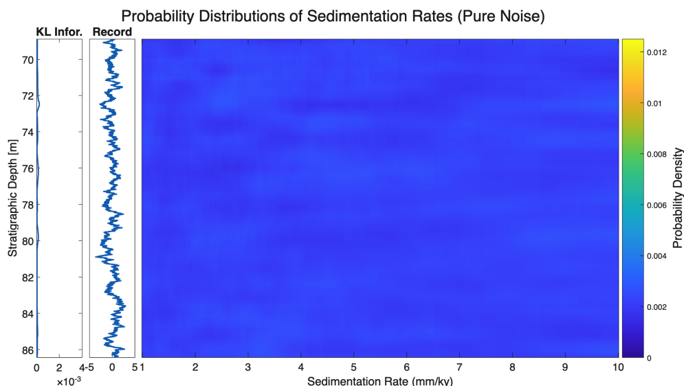
Figure 3. Probability density distributions of sedimentation rates computed from a pure noise signal (“Record” shown on the 2nd plot from left). Note the relative flatness of the posterior distributions, and the low values of the Kullback-Leibler information, relative to the synthetic data in Fig. 2.
