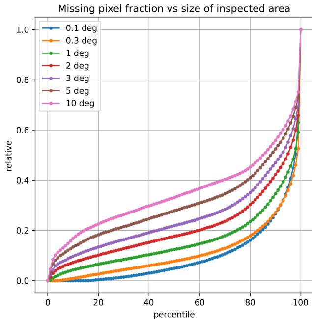
Figure 9. Distribution of mean fraction of MODIS missing pixels for different sizes of area around the detected fire inspected for presence of other fires. The green curve (1 deg area size) corresponds to panel (b) of Fig. 8. The curve 0.1 deg corresponds to no season checking, whereas the curve “10 deg” is practically equivalent to mean cloud fraction (Fig. 8a). Distribution is calculated only over land and regions with fires (Fig. 8b, c).
