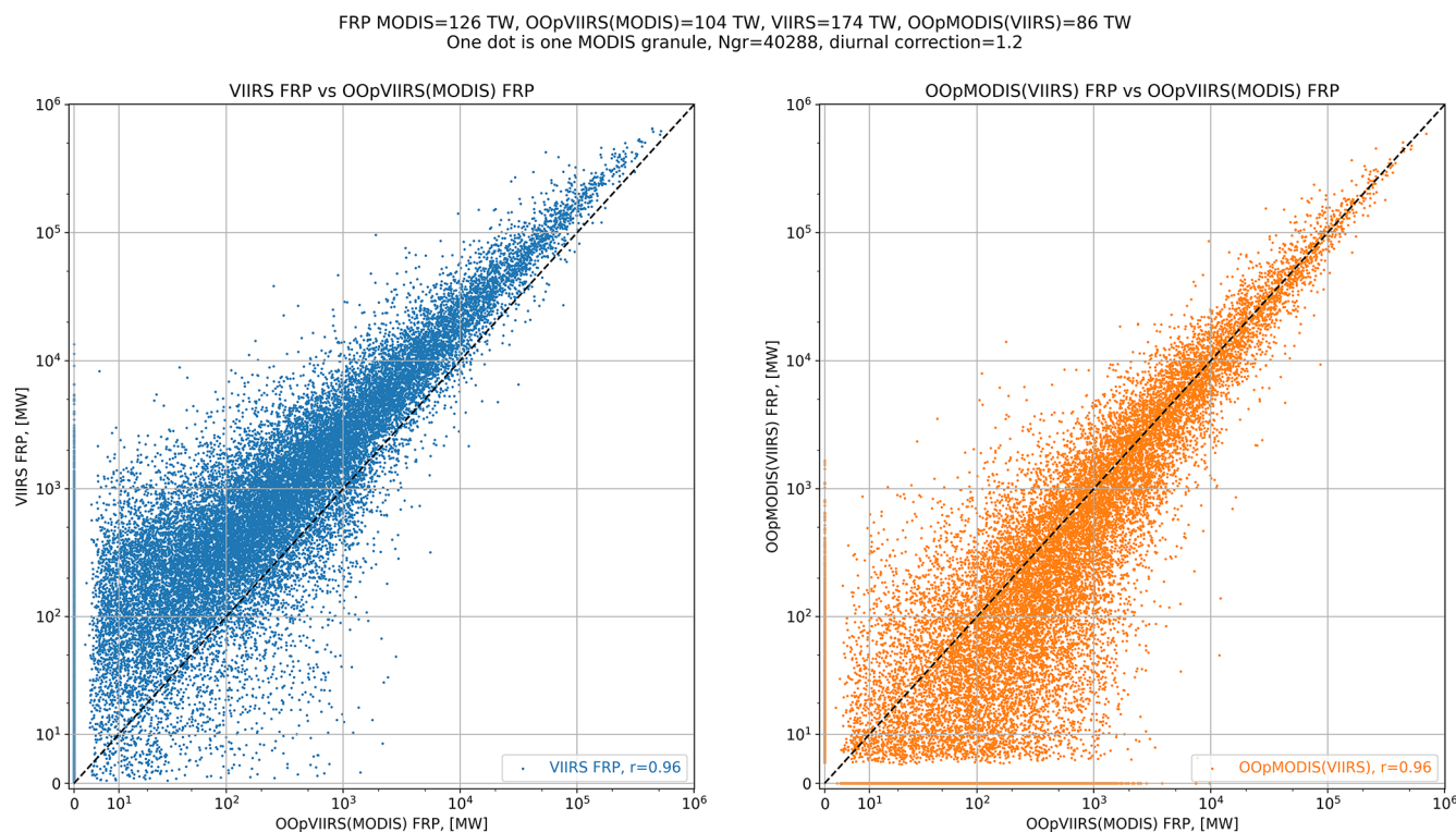
Figure 11. Summary of P_{\text{MODIS}} (blue) and \Xi_{\text{pixMODIS}}(P_{\text{VIIRS}}) (orange) for 2020. Each dot represents the total FRP of fires that fell to a single MODIS AQUA granule. Granules that did not have VIIRS coverage (missing or corrupted VIIRS granules) and granules with no fires in both instruments are filtered out. A diurnal variation correction factor 1.2 is applied to VIIRS retrievals (see Discussion section).
