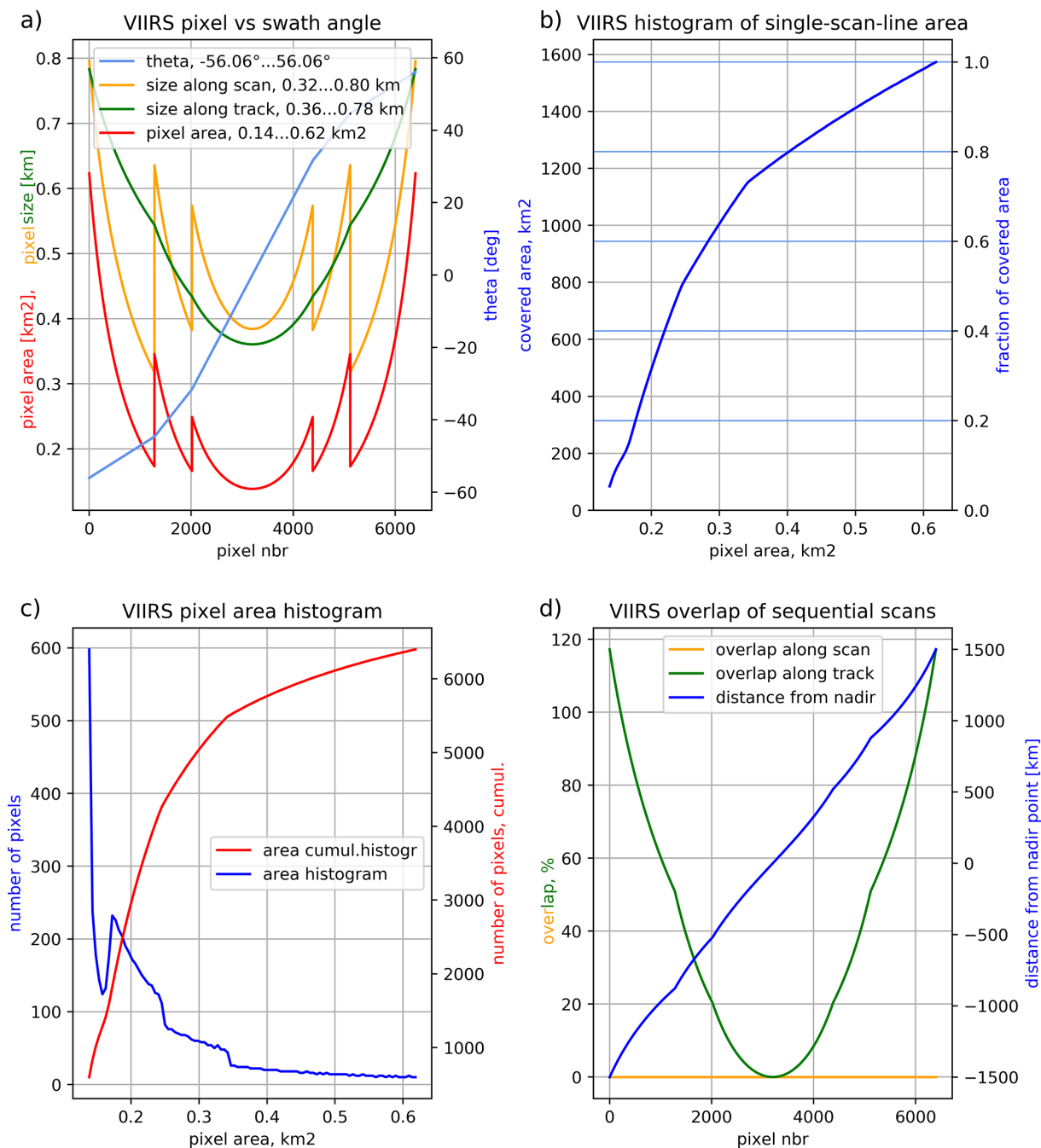
Figure 2. VIIRS swath geometry. Panels: (a) linear sizes, area, and viewing angle along the scan; (b) fraction of swath covered by pixels smaller than the given area; (c) distribution of pixel area; (d) overlap of pixels along the track and along the scan.
