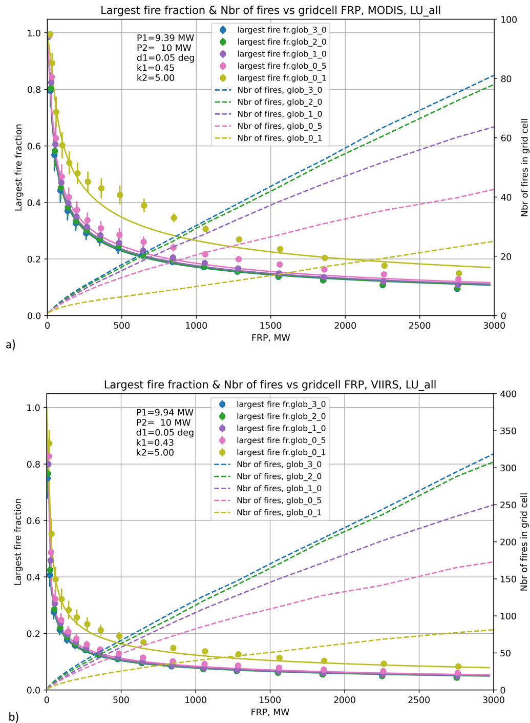
Figure 7. A mean fraction \gamma of the largest fire pixel in the total grid-cell FRP P , as a function of P . Calculated from MODIS 2000–2023 time series (a) and VIIRS 2018–2024 (b) as a function of grid-cell FRP for different grid resolutions dx . Fitting curves are computed from Eq. (8) with the coefficients shown at the plot. Charts and dots are slightly shifted horizontally to reduce overlapping.
