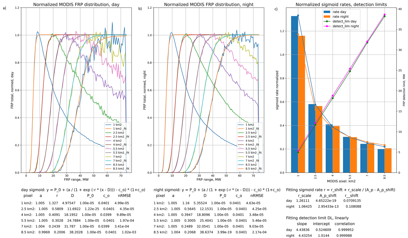
Figure 5. Definition of the detection limit as a function of pixel area via the normalized FRP distribution. Colored broken lines at panels (a) and (b) are the normalized vertical cross-sections of the panels (c) and (d) of Fig. 3, for day and night retrievals, respectively. All curves have been normalized to their smoothed max values. The rising part of each curve is approximated by a sigmoidal function with parameters shown under the panel. (c) Broken lines show FRP values corresponding to 0.5-level of the corresponding sigmoidal function of panels (a) and (b) – the detection limit for the specific pixel size; bars: slope of the sigmoid at those points.
