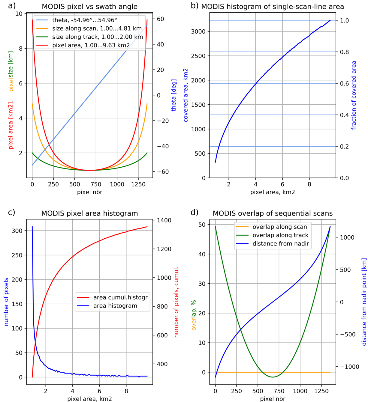
Figure 1. MODIS swath geometry. Panels: (a) linear sizes, area, and viewing angle along the scan; (b) fraction of swath covered by pixels smaller than the given area; (c) distribution of pixel area; (d) overlap of pixels along the track and along the scan.
