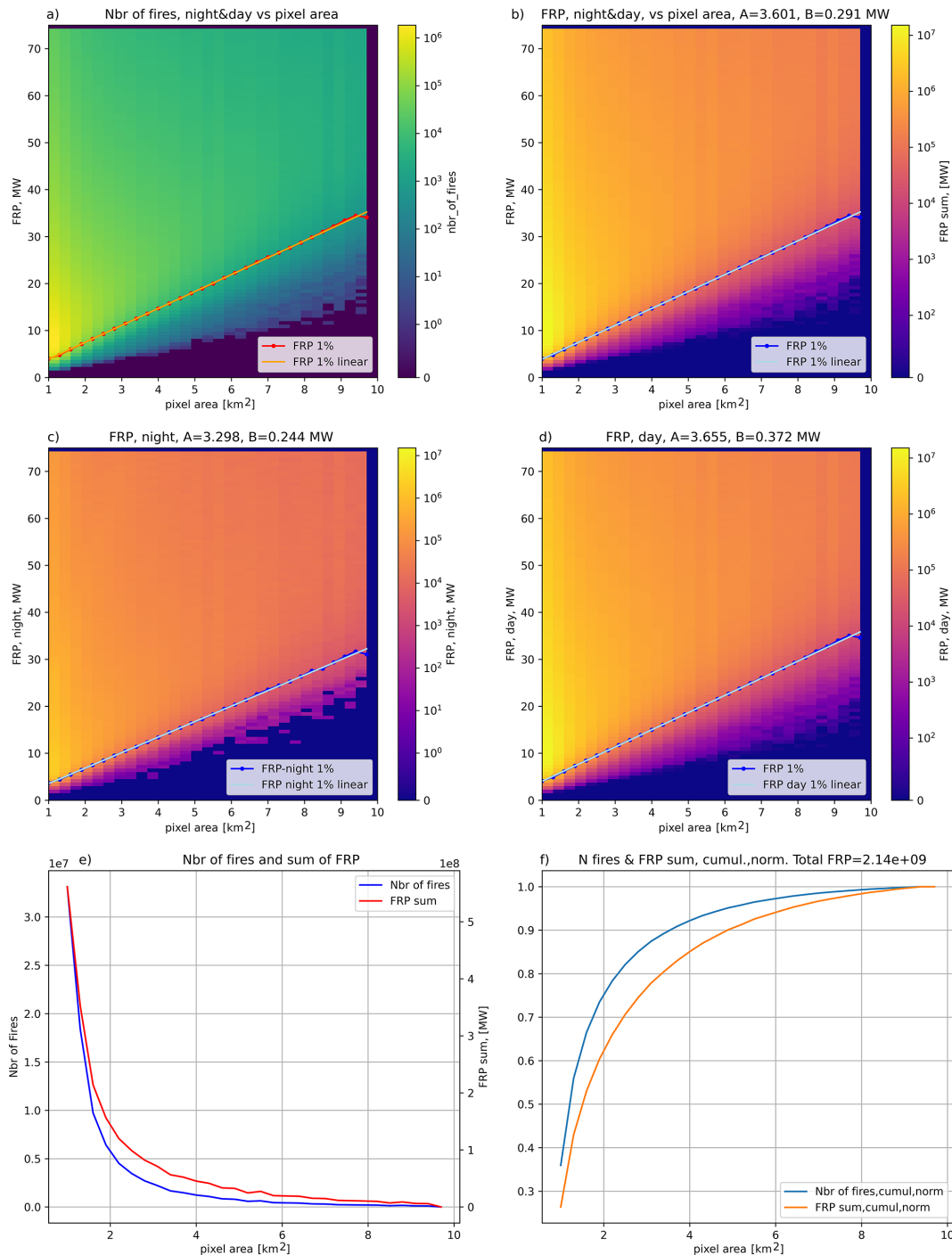
Figure 3. Distribution of the fire pixels detected by MODIS below 75 MW (arbitrarily taken cut-off allowing to see the peaks of the distributions and detection limits) as a function of a pixel size and FRP. Panel (a) Total number of fire pixels for all overpasses, (b) Total FRP of all overpasses, (c) Total FRP registered by night-time overpasses; (d) Total FRP registered by day-time overpasses; (e) Total FRP and number of fire pixels of the specific area, all FRP values counted (no upper limit); (f) same as (e) but cumulative. (a–d) Red dots represent the 1 %-tile for each pixel area whereas the orange lines on top of them represent the corresponding linear approximations, which slope A and intercept B are shown in the panel titles.
