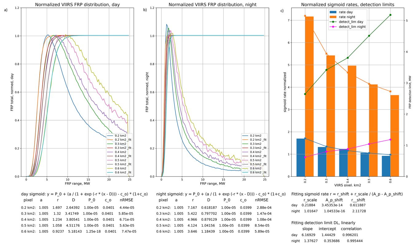
Figure 6. Definition of the FRP detection limit as a function of pixel size via the normalized FRP distribution for VIIRS. Panels are the same as in Fig. 5. Colored broken lines at panels (a) and (b) are the normalized vertical cross-sections of the panels (c) and (d) of Fig. 4 for day and night retrievals, respectively. All curves have been normalized to their smoothed max values. The rising part of each curve is approximated by a sigmoid function with parameters shown under the panel. (c) Broken lines: FRP values corresponding to 0.5 levels of the corresponding sigmoid function of panels (a) and (b) – the detection limit for the specific pixel size; bars: slope of the sigmoid at those points.
