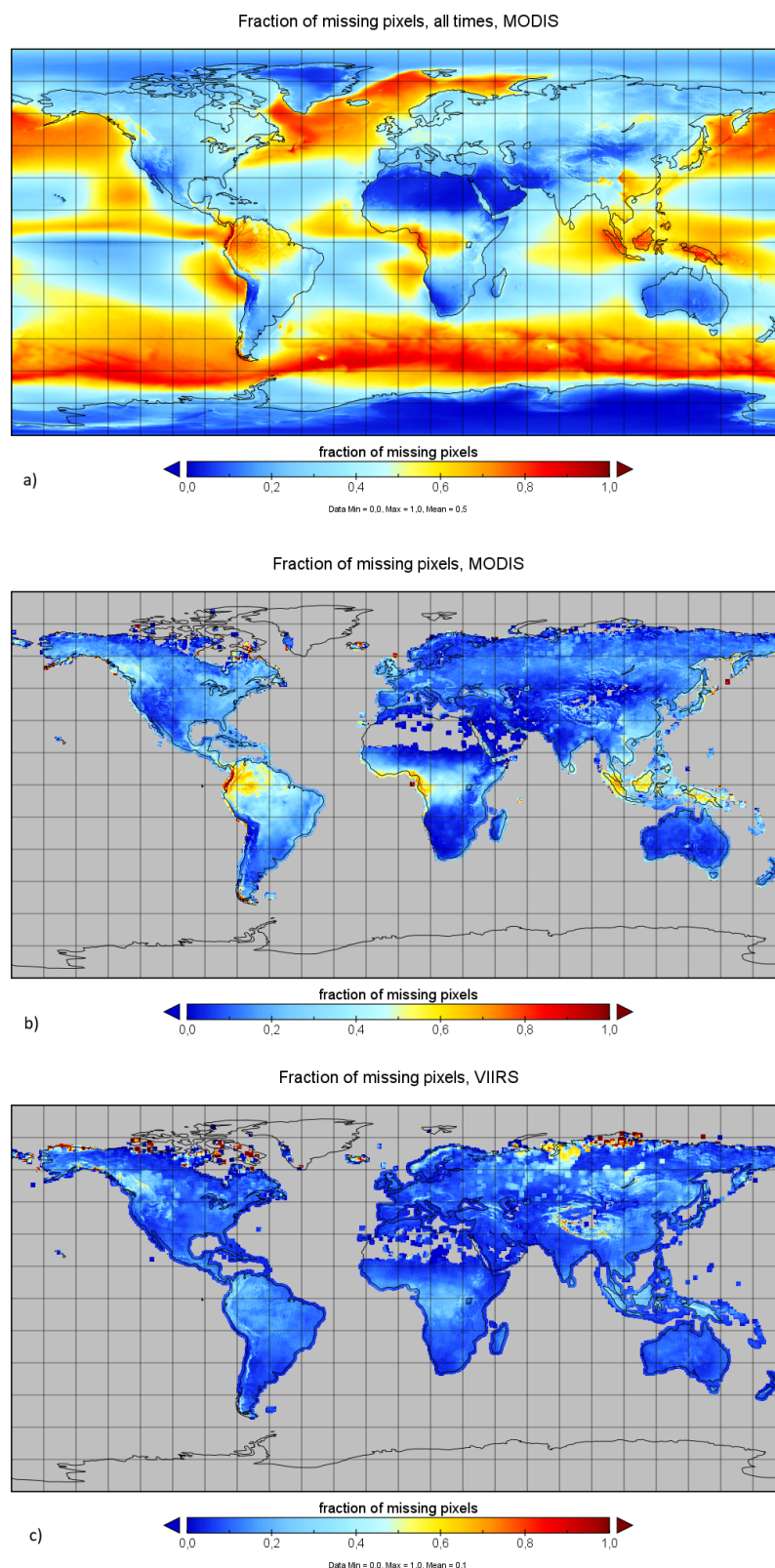
Figure 8. Mean fraction of missing pixels due to cloud obscuration of MODIS, 2000–2020, and VIIRS, 2018–2024. Panel (a) mean over all MODIS overpass times, (b) mean over hours when non-zero FRP registered by MODIS anywhere in 1^\circ \times 1^\circ square centered around the grid cell, (c) mean over hours when non-zero FRP registered by VIIRS anywhere in 1^\circ \times 1^\circ square centered around the grid cell.
