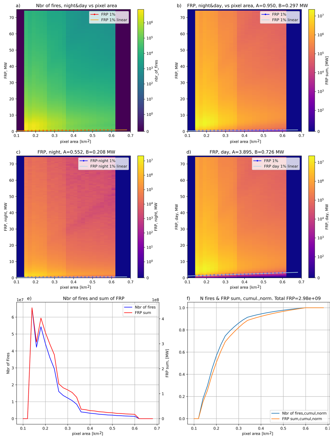
Figure 4. Distribution of the fire pixels detected by VIIRS as a function of the pixel area and FRP. Same panels as for Fig. 3. Panel (a) Total number of fires for all overpasses, (b) Total FRP of all overpasses, (c) Total FRP registered by night-time overpasses; (d) Total FRP registered by day-time overpasses; (e) Total FRP and the number of fires registered by the pixels of the specific size, all FRP values counted (no upper limit); (f) same as (e) but cumulative. (a–d) Red dots represent the 1 %-tile for each pixel area whereas the orange lines on top of them represent the corresponding linear approximations, which slope A and intercept B are shown at the panel titles.
