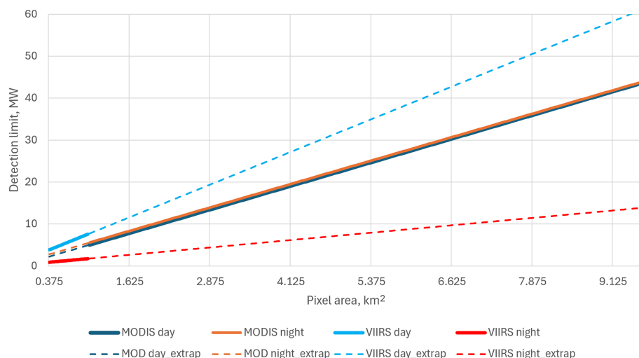
Figure 12. MODIS and VIIRS detection limits as functions of pixel sizes. Solid lines denote the actual pixel size range of the instruments, whereas dashed lines show their extrapolation to cover the whole size range 0.375–9.6 km 2 .
