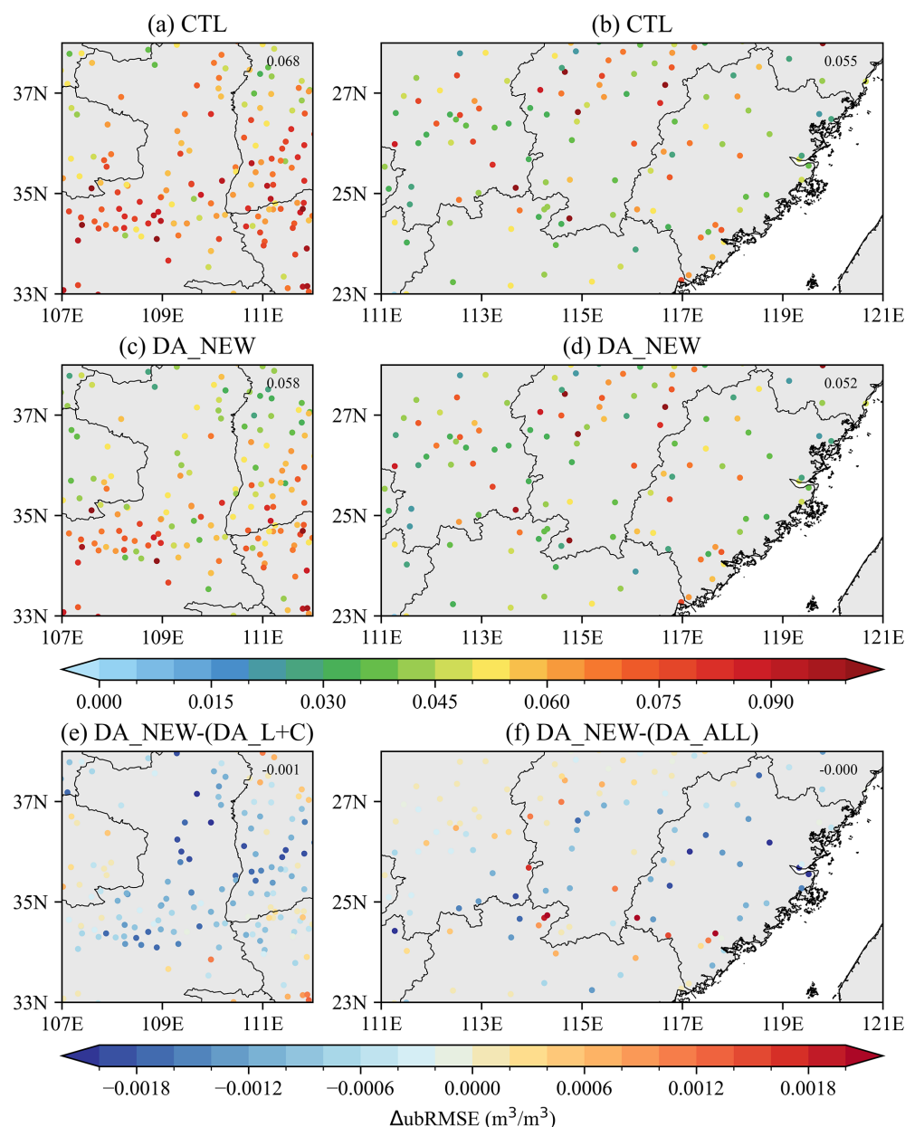
Figure 17. Same as Fig. 16 except for ubRMSE.
