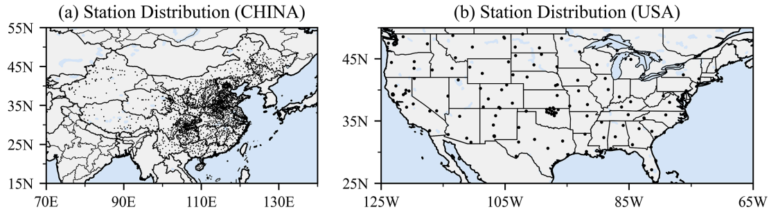
Figure 2. Spatial distribution of the in-situ soil moisture stations. (a) China Meteorological Administration network, and (b) International Soil Moisture Network stations located in the United States.
