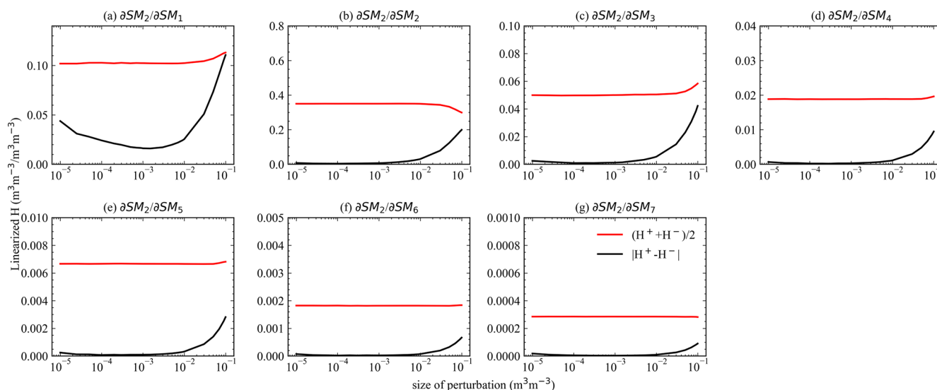
Figure 3. The \partial SM_2 / \partial SM_n characteristics with respect to size of perturbation in different layers are shown. The black line represents |H^+ - H^-| , and the red line represents (H^+ + H^-)/2 .
