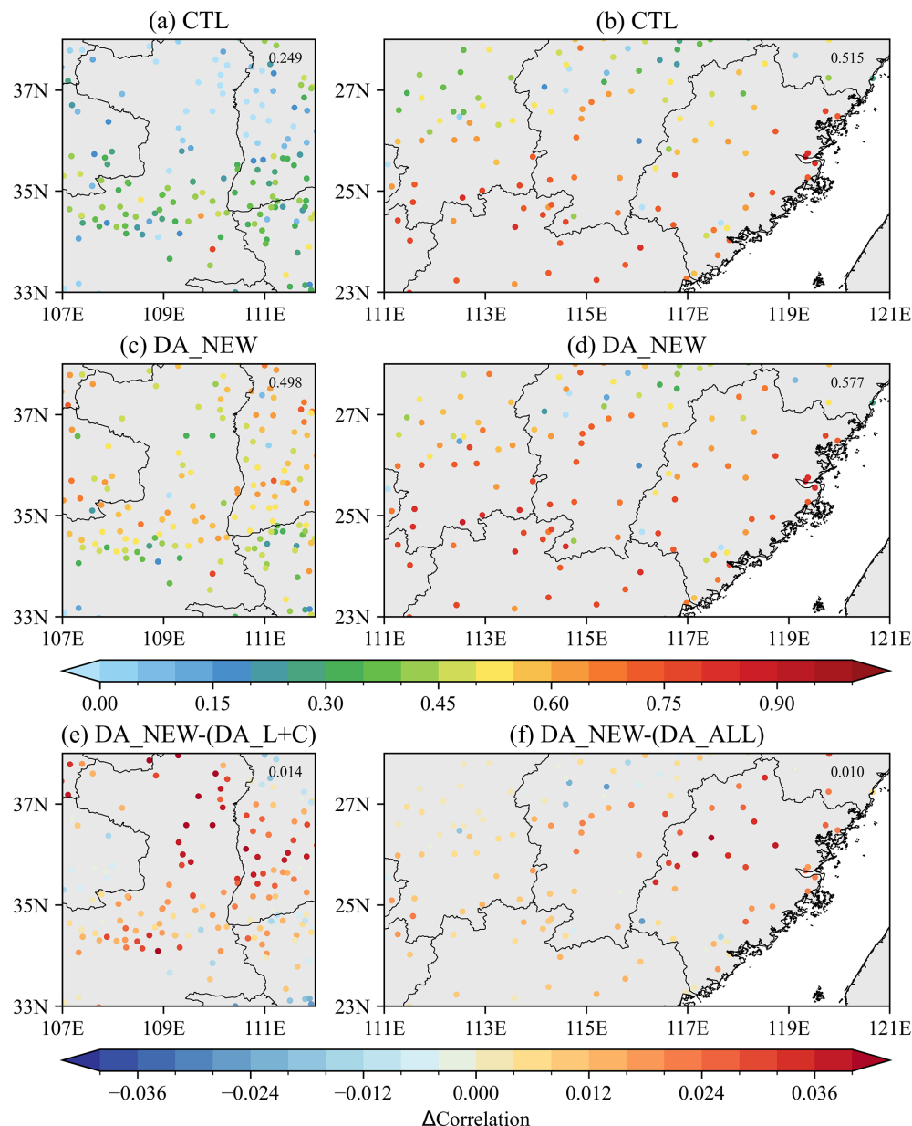
Figure 16. Spatial distribution of correlation coefficients between simulated and observed soil moisture. (a, b) show CTL results for central-west and southeast China, respectively, (c, d) show NEW experiment results for central-west and southeast China, respectively, and (e, f) show correlation differences between the NEW experiment and DA_L+C and between the NEW experiment and DA_ALL, respectively.
