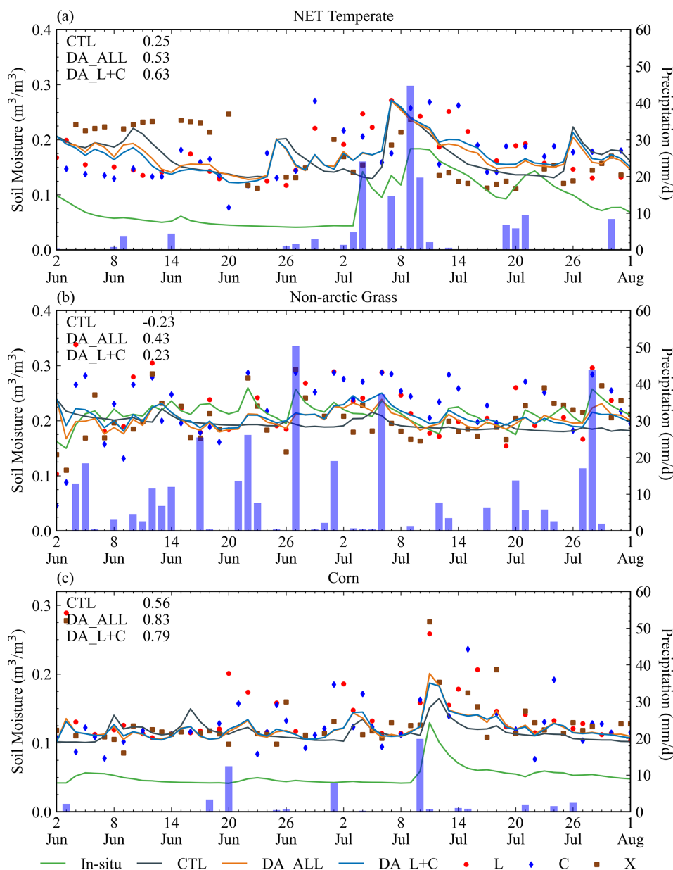
Figure 14. Time series of daily mean soil moisture from model simulations, satellite retrievals, and in situ observations for different assimilation experiments. The green solid line represents in situ observations. Black, orange, and blue solid lines indicate soil moisture simulations from the control experiment, the DA_ALL assimilation experiment, and the DA_L+C assimilation experiment, respectively. Red dots, blue diamonds, and brown squares represent L- (SMAP), C- (ASCAT), and X-band (MWRI) satellite soil moisture products, respectively. Blue bars denote daily precipitation.
