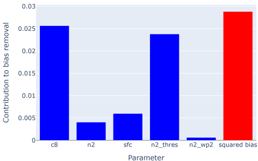
Squared parameter contributions to bias removal
