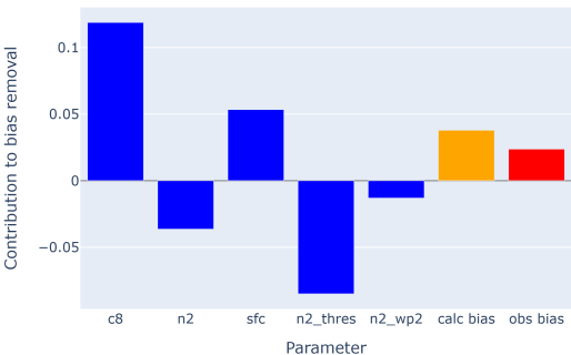
Mean parameter contributions to removal of biases
