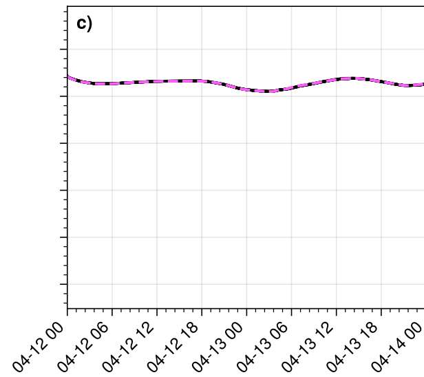
OIFS 43r3 – NEMO 4.0.1
