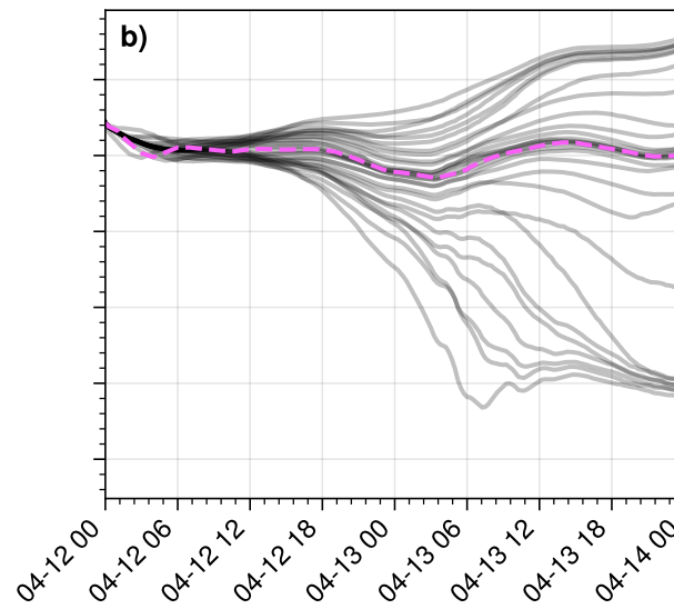
OIFS 43r3 – NEMO 3.6
