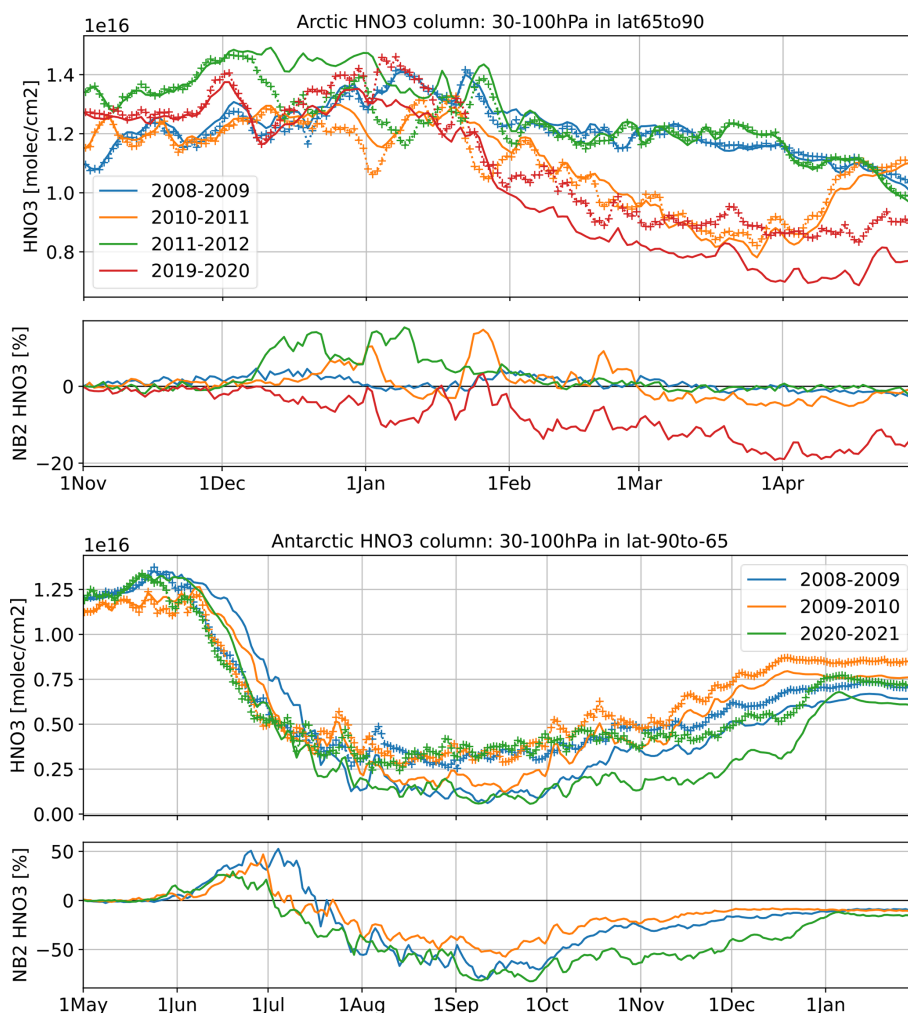
Figure 12. Same as Fig. 11 but for \text{HNO}_3 .
