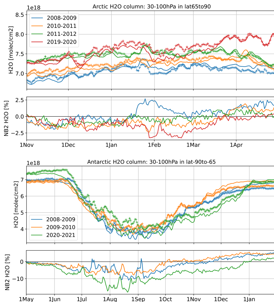
Figure 11. A time series of the H 2 O partial columns (30–100 hPa, upper panels) in IFS-COMPO Cy49R1 chemical forecasts (solid lines) and in the BRAM3 reanalysis (crosses), and the corresponding normalized biases (lower panels). Comparisons are shown for both the Arctic (65–90° N, top) and the Antarctic (90–65° S, bottom) for the same years and using the same color scheme as in Fig. 3.
