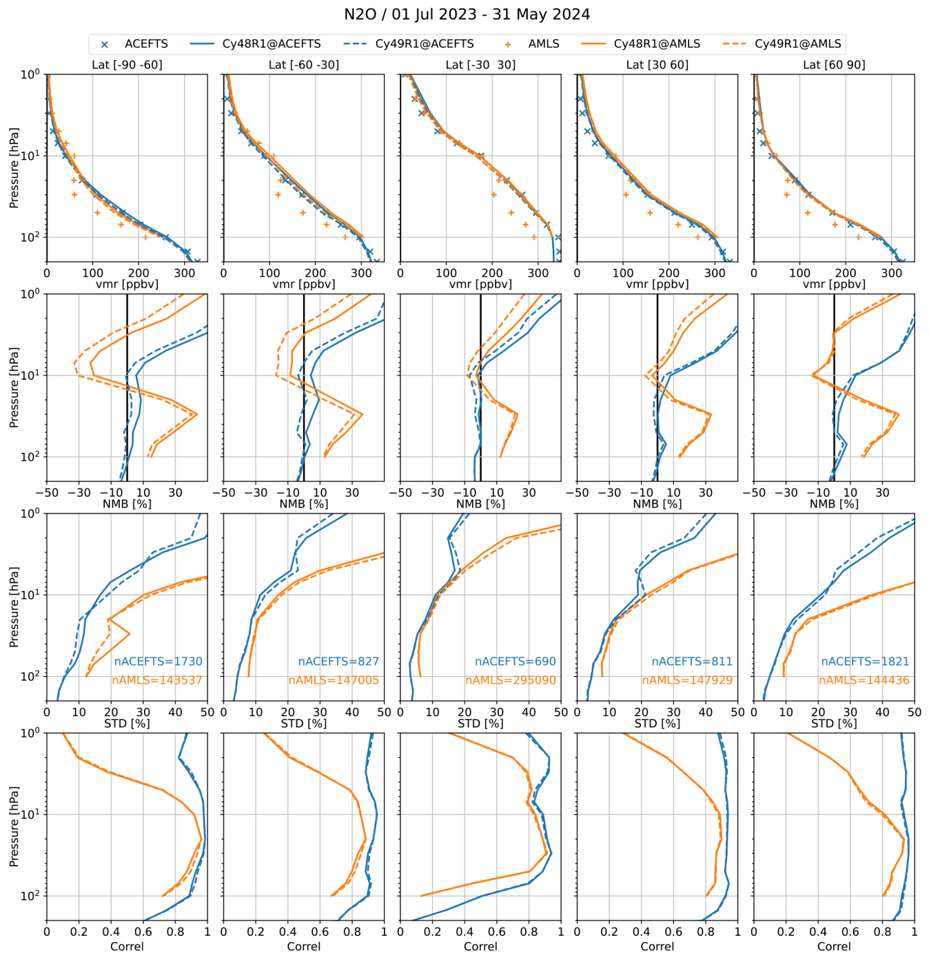
Figure 4. Comparison of N 2 O simulated in the IFS-COMPO control runs Cy48R1 (solid lines) and Cy49R1 (dashed lines) with MLS (orange) and ACE-FTS (blue) profile observations between July 2023 and May 2024. Statistics are segregated into five latitude bands spanning both the Southern and Northern Hemispheres, from left to right: 90–60° S, 60–30° S, 30° S–30° N, 30–60° N and 60–90° N. Statistical values shown are, from top to bottom: mean volume mixing ratio (vmr); mean bias (model minus observations) normalized by the mean of the model profile (NMB); standard deviation of the mean bias (STD); and the correlation between models and observations (Correl). The number of profiles used in each comparison are given in the third (STD) row.
