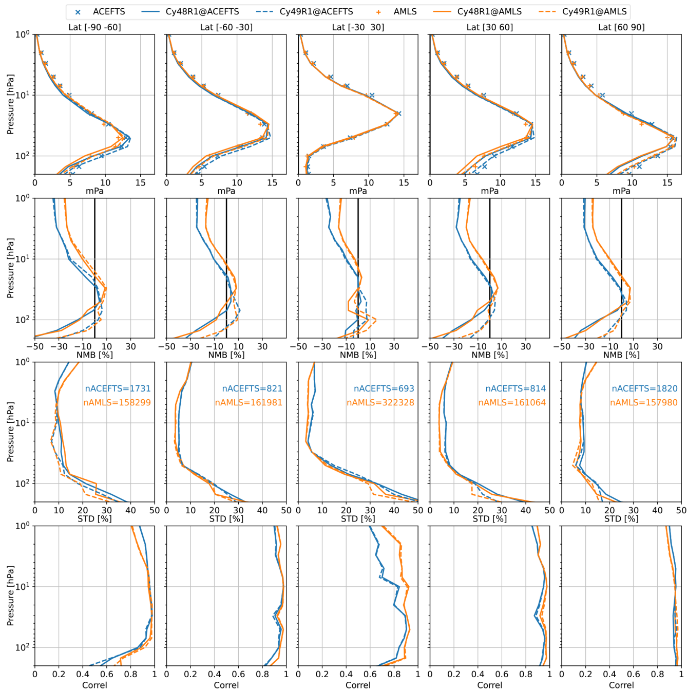
Figure 9. Same as Fig. 4 but for O 3 with the top row showing partial pressures in mPa.
