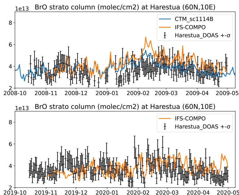
Figure 16. A time series of the stratospheric BrO Vertical Column Density above Harestua (60.2° N, 10.8° E) during the 2008–2009 (top) and 2019–2020 (bottom) winter-spring seasons. Black symbols and error bars: UV-Vis DOAS retrievals adjusted to 13:30 LT with a box-model; solid lines: results by IFS-COMPO Cy49R1 (orange) and by the BASCOE CTM with an updated chemical scheme (blue, 2008–2009 only) at noon UT.
