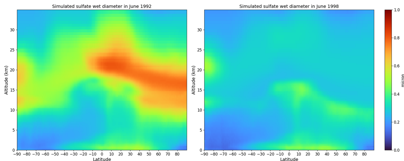
Figure 2. Altitude-latitude monthly-mean cross sections of sulfate wet diameter ( \mu\text{m} ) as simulated by IFS-COMPO Cy49R1 in June 1992 (left, representative of volcanic conditions), and June 1998 (right, representative of quiescent conditions).
