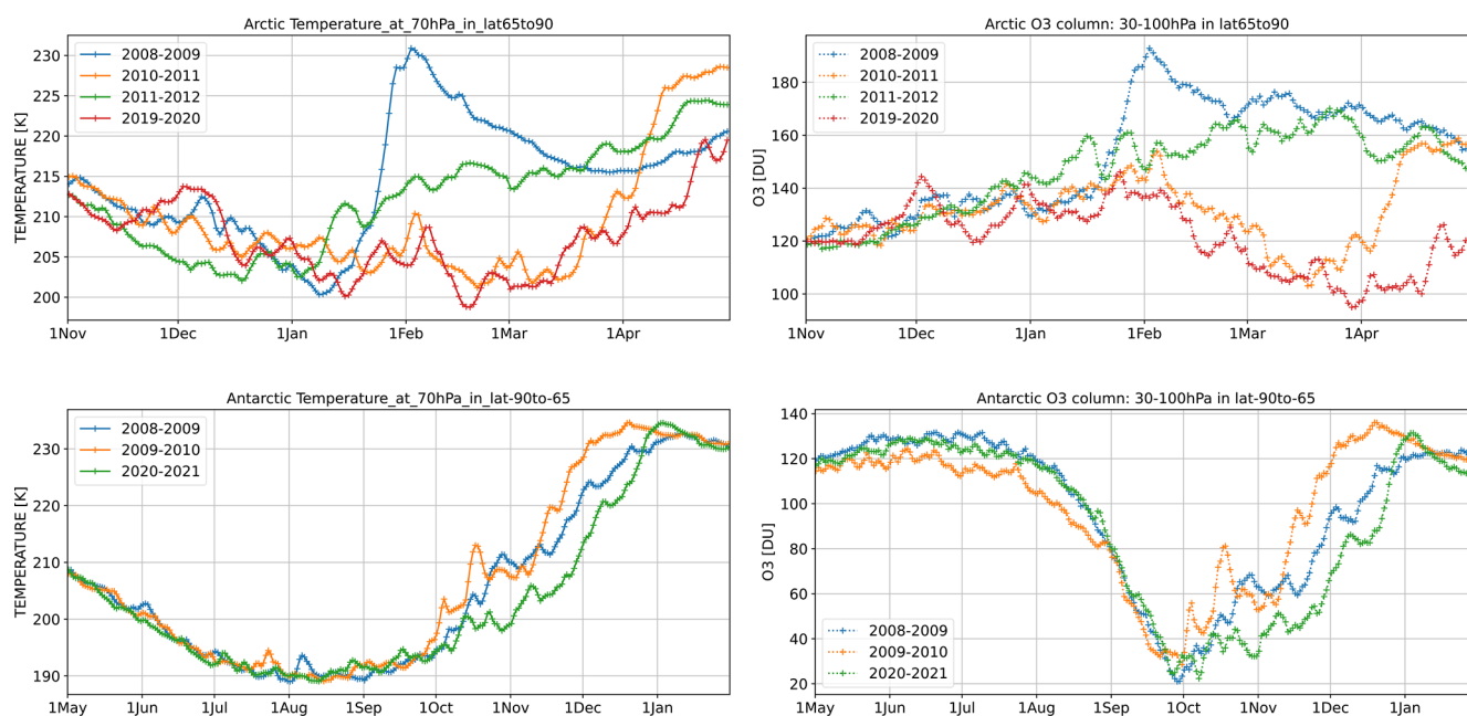
Figure 3. Mean ERA5 temperature at 70 hPa (left) and BRAM3 reanalyses of the \text{O}_3 partial columns (30–100 hPa, right) above the Arctic (65–90° N, top) for the winter-spring seasons of 2008–2009 (blue), 2010–2011 (orange), 2011–2012 (green) and 2019–2020 (red) and above the Antarctic (90–65° S, bottom) for the winter-spring seasons of 2008 (blue), 2009 (orange) and 2020 (green).
