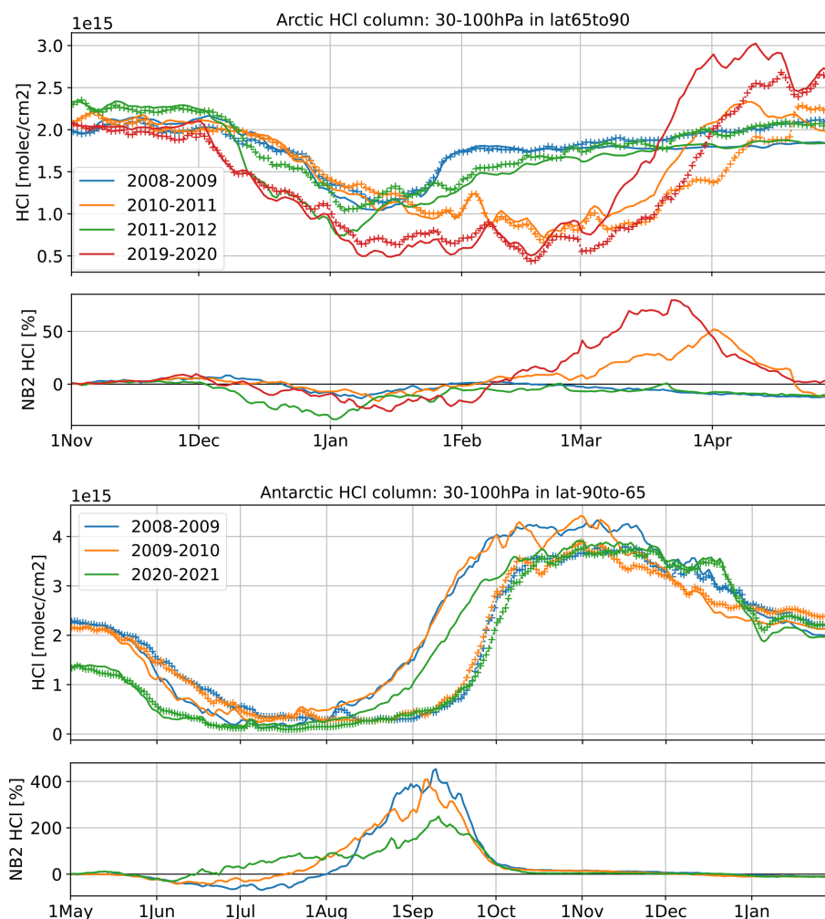
Figure 13. Same as Fig. 11 but for HCl.
