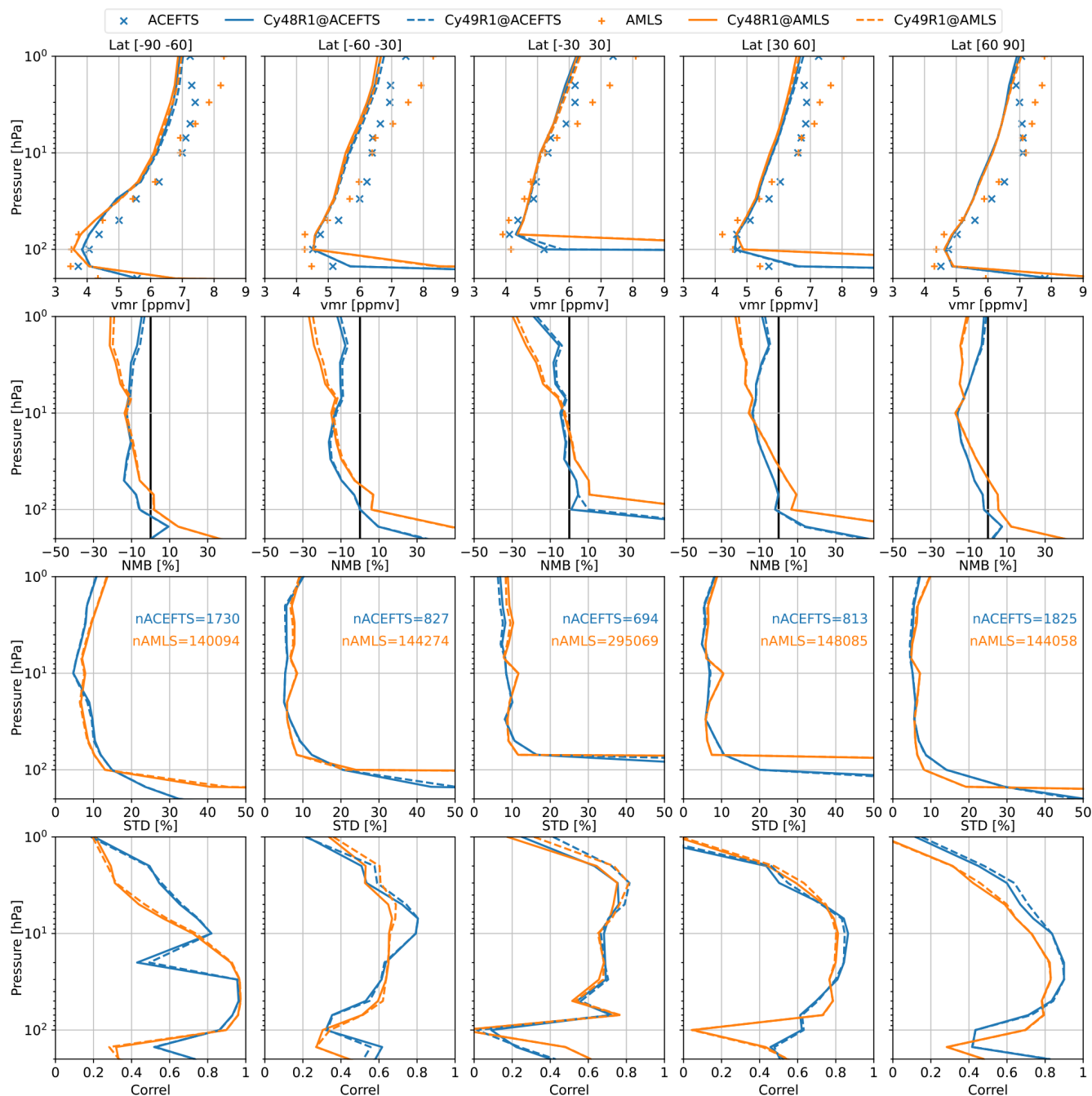
Figure 5. Same as Fig. 4 but for H 2 O.
