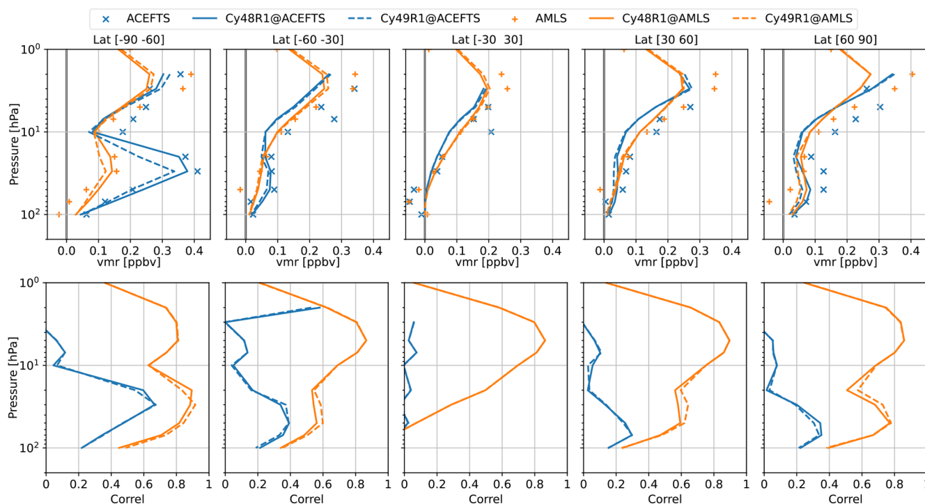
Figure 7. Same as Fig. 4 but for CIO and showing only the volume mixing ratios and correlations. The number of profiles used in each comparison are nearly identical with those used for HCl (see previous Figure).
