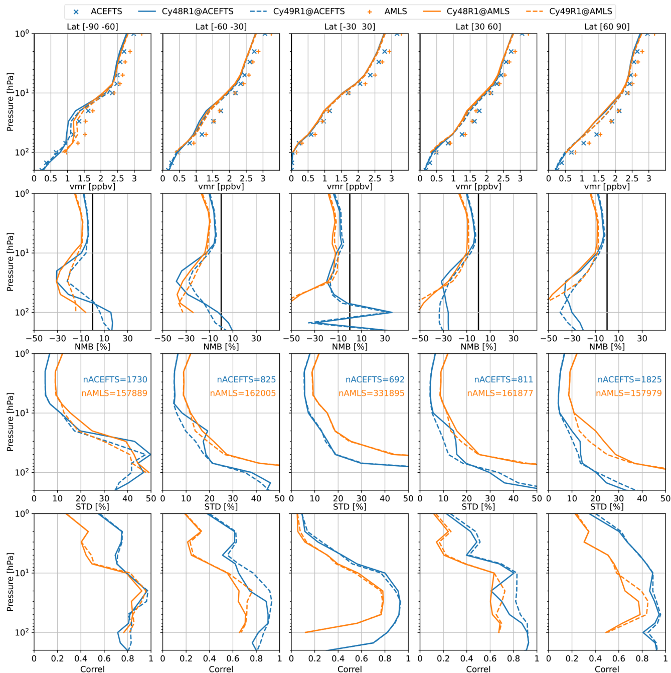
Figure 6. Same as Fig. 4 but for HCl.
