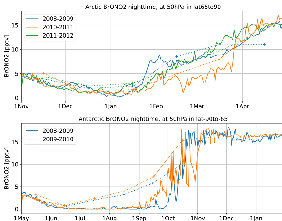
Figure 17. Same as Fig. 15 but for nighttime (i.e., solar zenith angle > 90^\circ ) BrONO 2 volume mixing ratios at the 50 hPa pressure level, using MIPAS monthly means as references (dotted lines; Höpfner et al., 2021).
