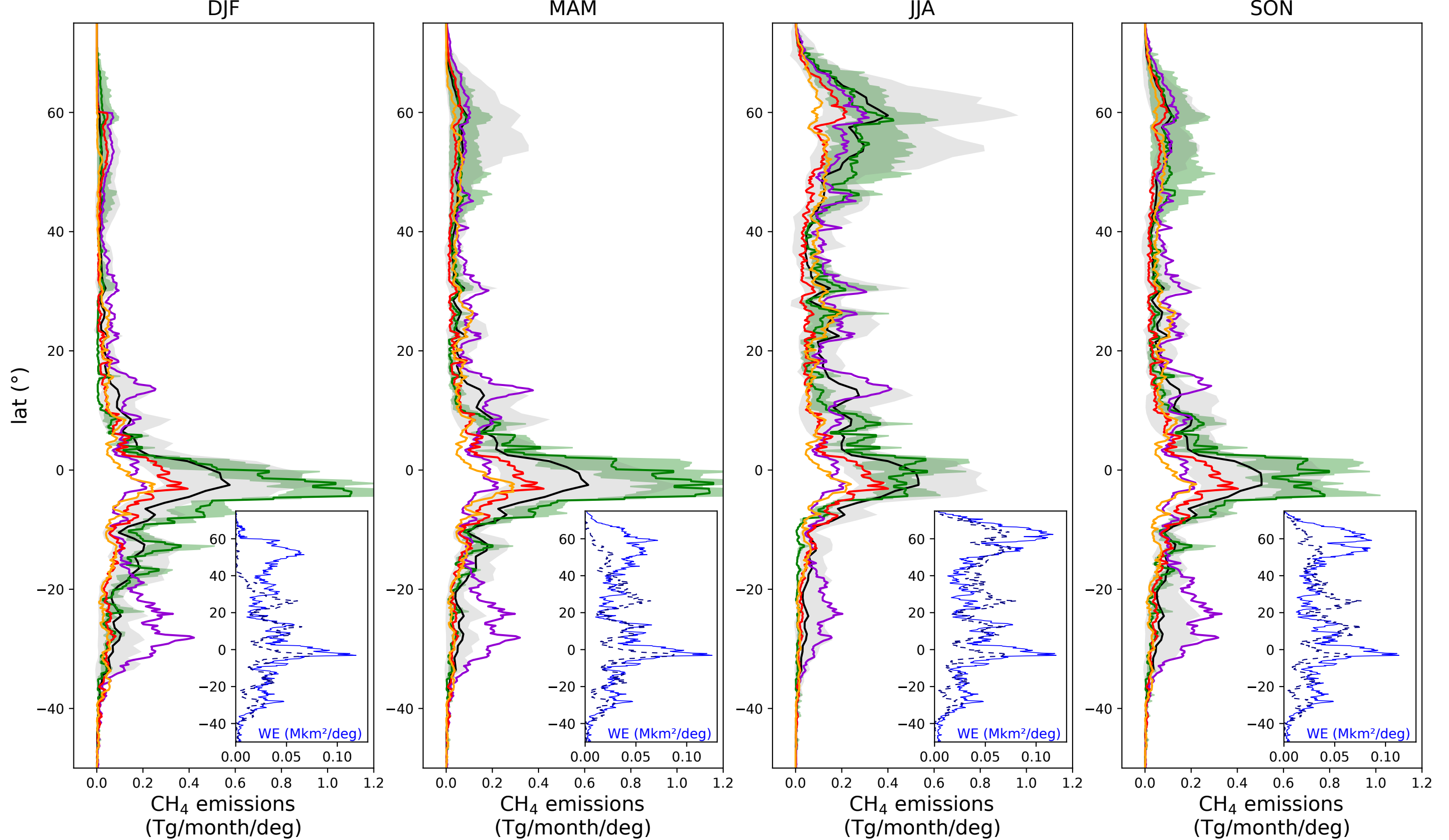
— This study - WAD2M — GMB model diagnostic mean — WetCHARTs 166Tg/yr models mean — UpCH 4 - WAD2M — WAD2M — This study - TOPMODEL GMB diagnostic ensemble WetCHARTs 166Tg/yr models - - - TOPMODEL
