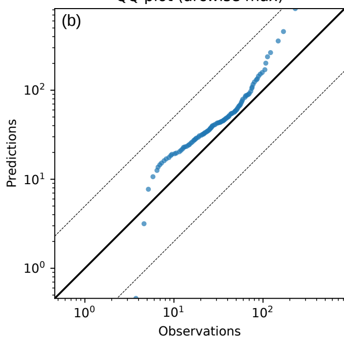
QQ plot (arcwise max)
