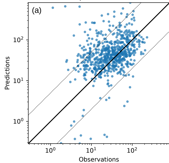
Scatter plot (arcwise max)
