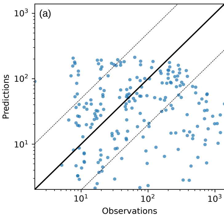
Scatter plot
