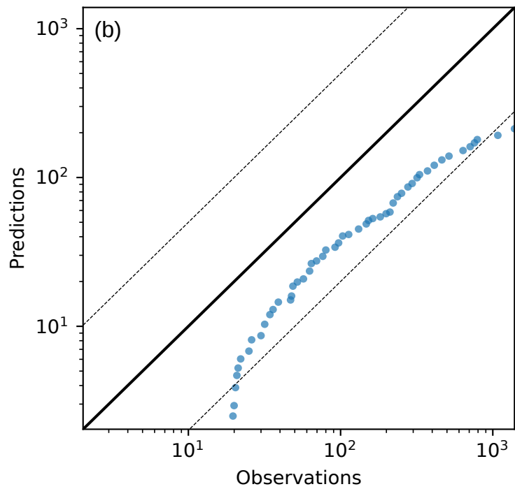
QQ plot
