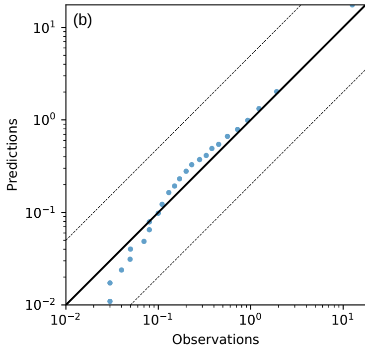
QQ plot
