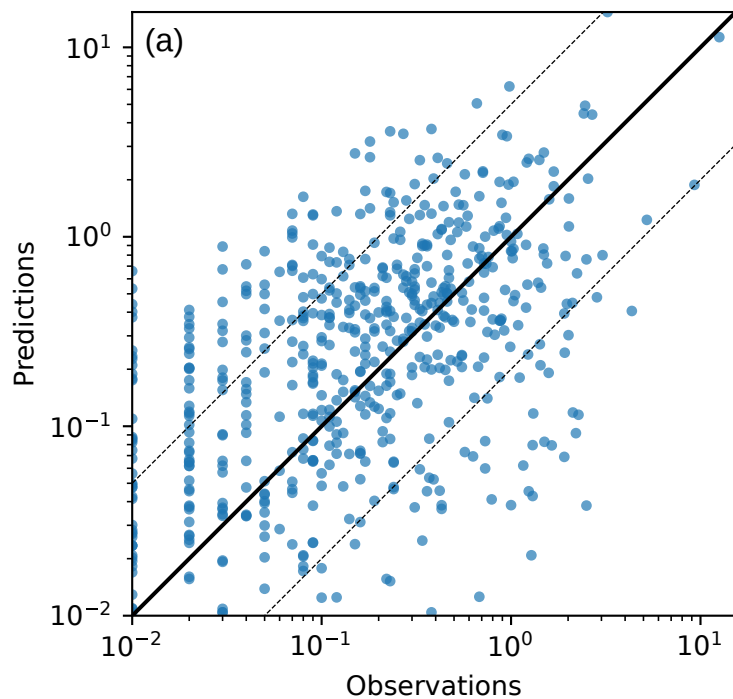
Scatter plot
