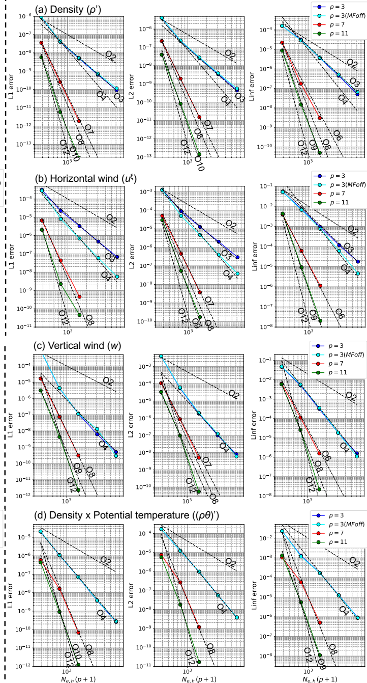
Case of analytical Jacobian cofactor
