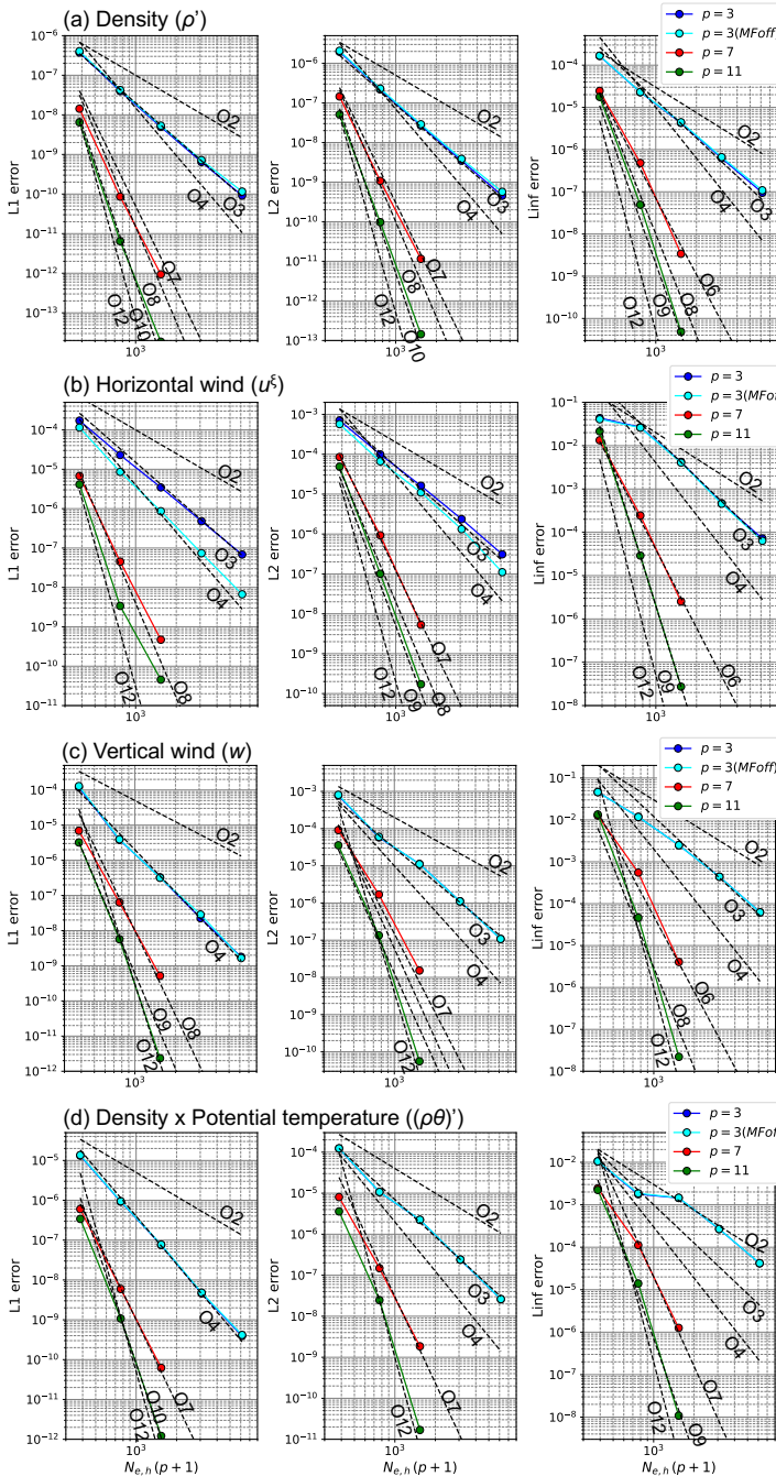
Case of numerically calculated Jacobian cofactor
