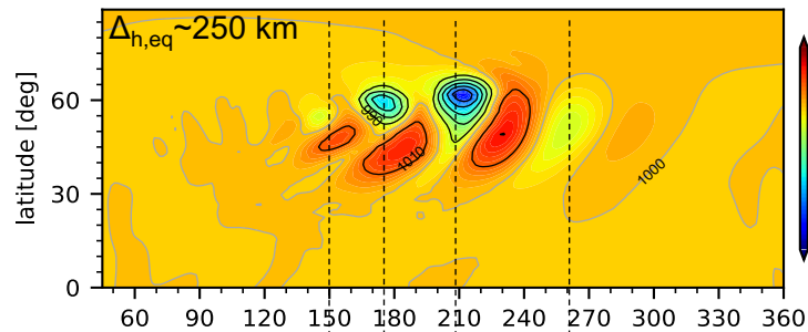
(a) Surface pressure [hPa]
