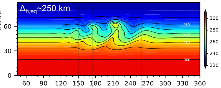
(b) Temperature at 850 hPa [K]
