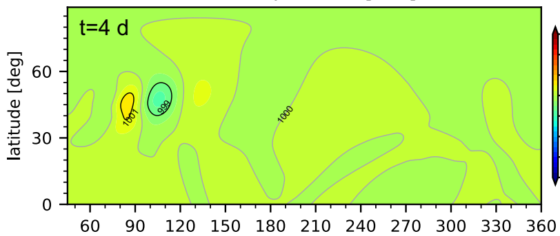
Surface pressure [hPa]
