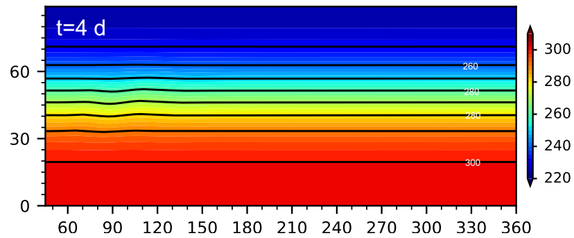
Temperature at 850 hPa [K]
