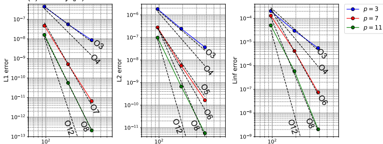
(b) Horizontal wind ( u^{\delta} )
