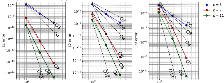
(c) Vertical wind ( w )
