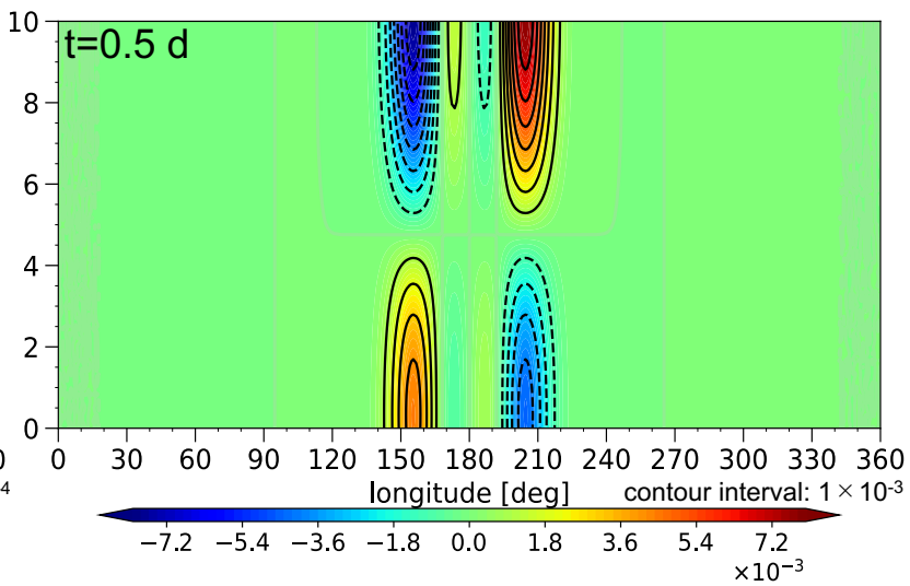
Zonal wind [m/s]
