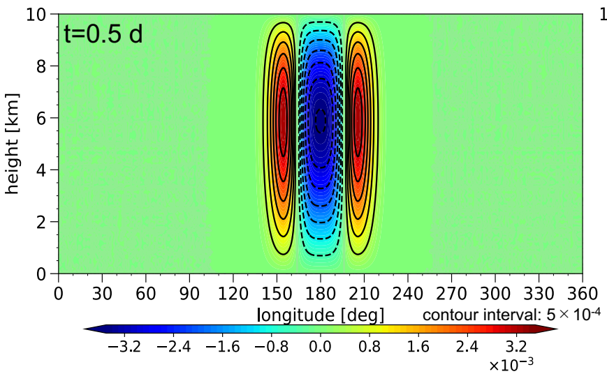
Potential temperature perturbation [K]
