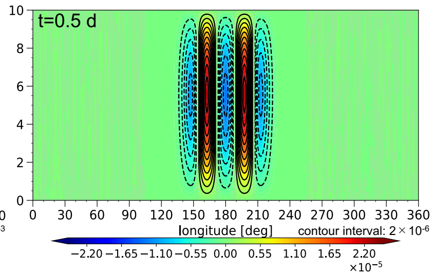
Vertical wind [m/s]
