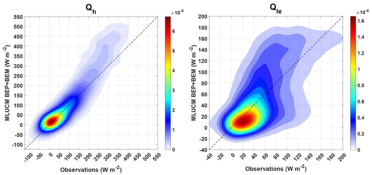
Figure S1: As in Figure 3, but during daytime (i.e. shortwave downward radiation > 10 W m -2 ).
