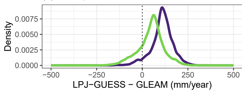
(e) Soil evaporation
