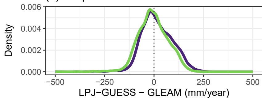
(c) Transpiration
