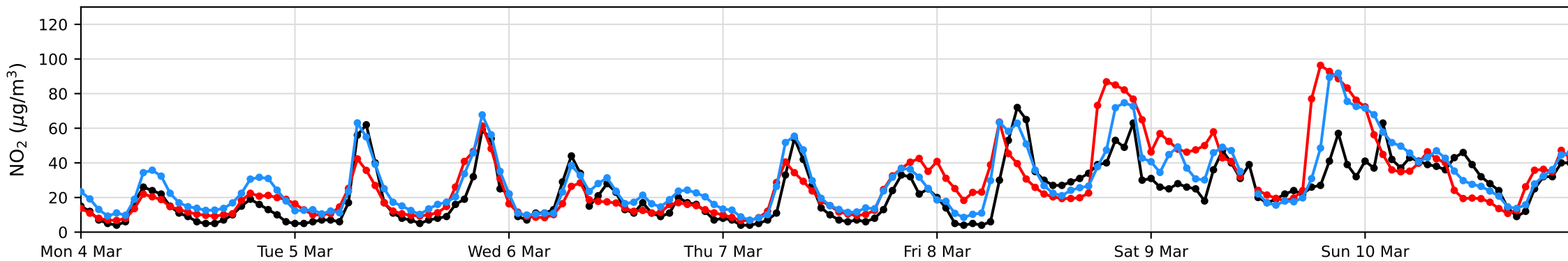
NO 2 concentrations at Casa de Campo (ES1193), suburban background
