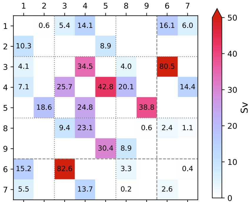
IPSL-CM5A2 Pre-Ind. GEOCLIM
