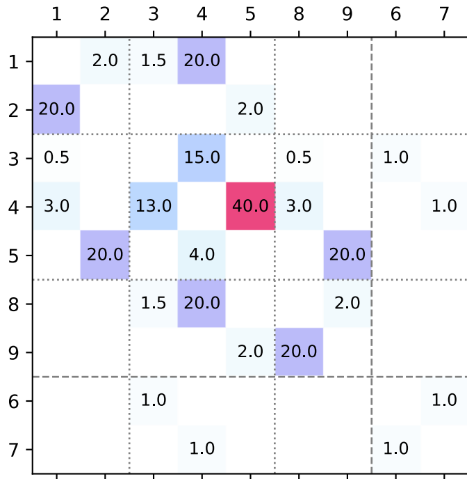
"historical" Pre-Ind. GEOCLIM
