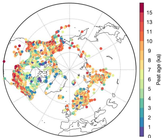
Figure S1: Spatial distribution of peat initiation age over 2,860 peat cores obtained from Loisel et al. (2017). The spatial extent of the map covers 30°N-90°N.
