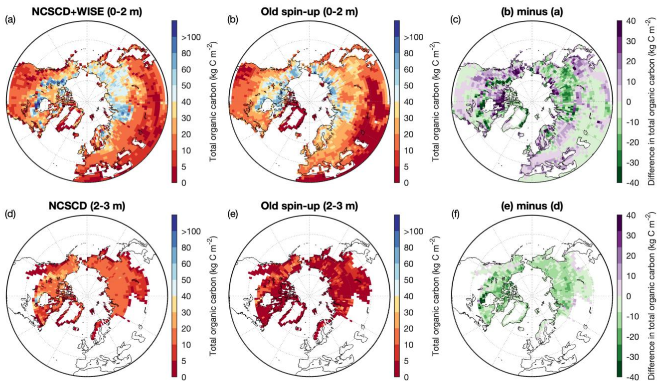
35 Figure S7: Same as Fig. 8, but for comparison of total organic carbon between the old spin up simulation and observation-based datasets.
