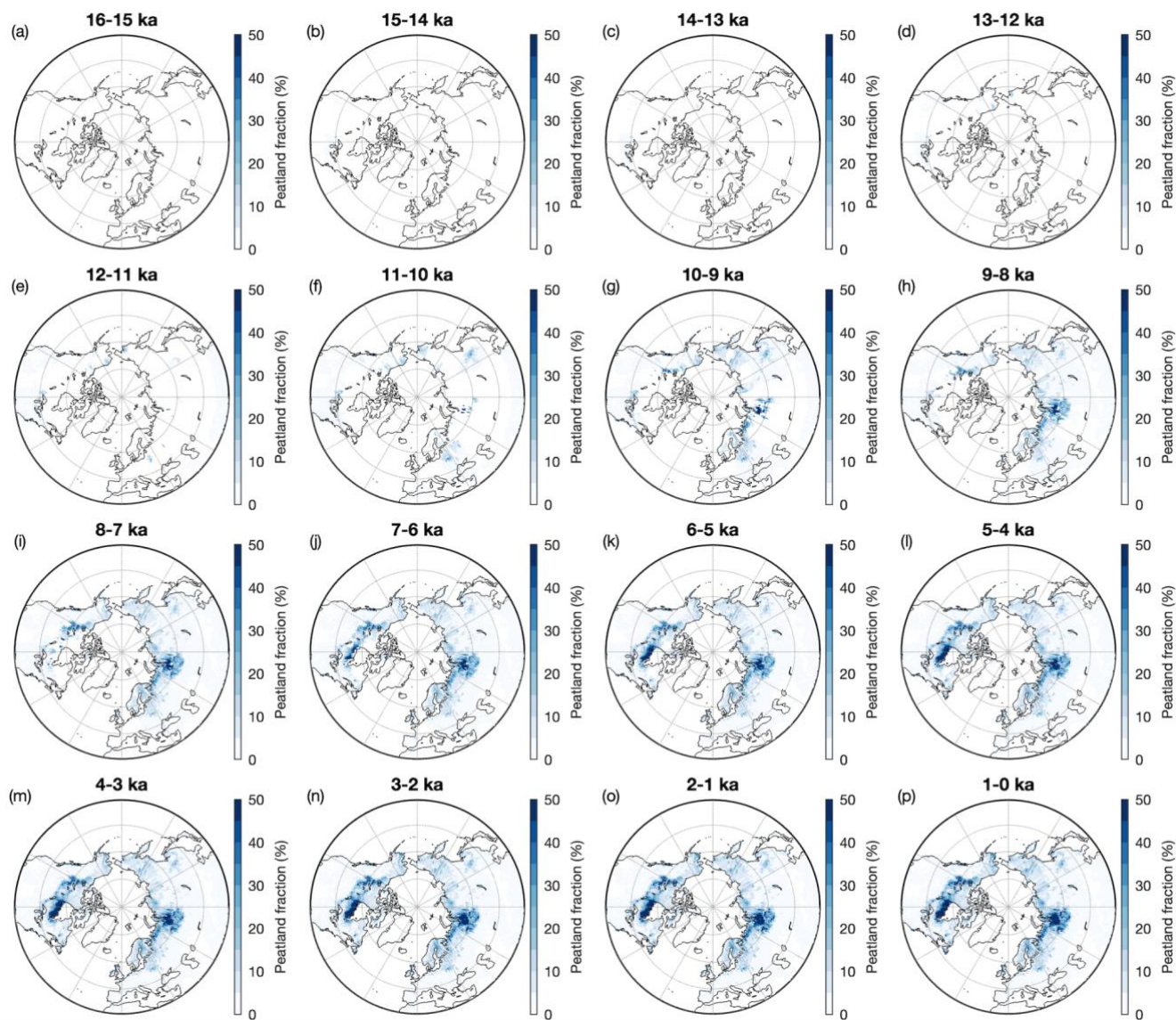
Figure S2: Spatial distribution of northern peatlands during each thousand-year from 16 ka to present. The spatial resolution is at 1^\circ \times 1^\circ , covering 30^\circ\text{N} - 90^\circ\text{N} .
