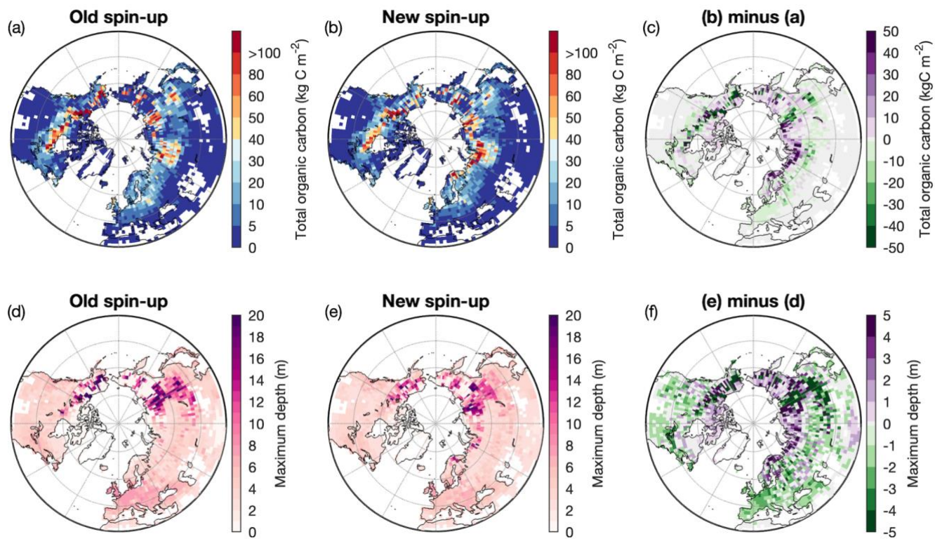
Figure S5: Same as Fig. 7, but for the total organic carbon and the maximum depth of soil organic carbon for peat PFT. To compare with Fig. 7, the unit for total organic carbon uses per m 2 grid cell.
