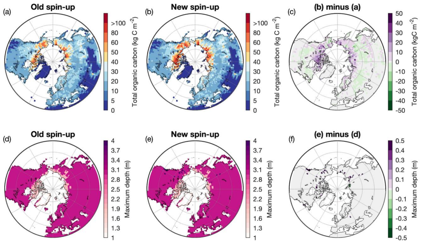
Figure S4: Same as Fig. 7, but for the total organic carbon and the maximum depth of soil organic carbon for 15 conventional PFTs. To compare with Fig. 7, the unit for total organic carbon uses per m 2 grid cell. Please note that the scale for the maximum depth of soil organic carbon in this figure is different from Fig. 7 and Fig. S5.
