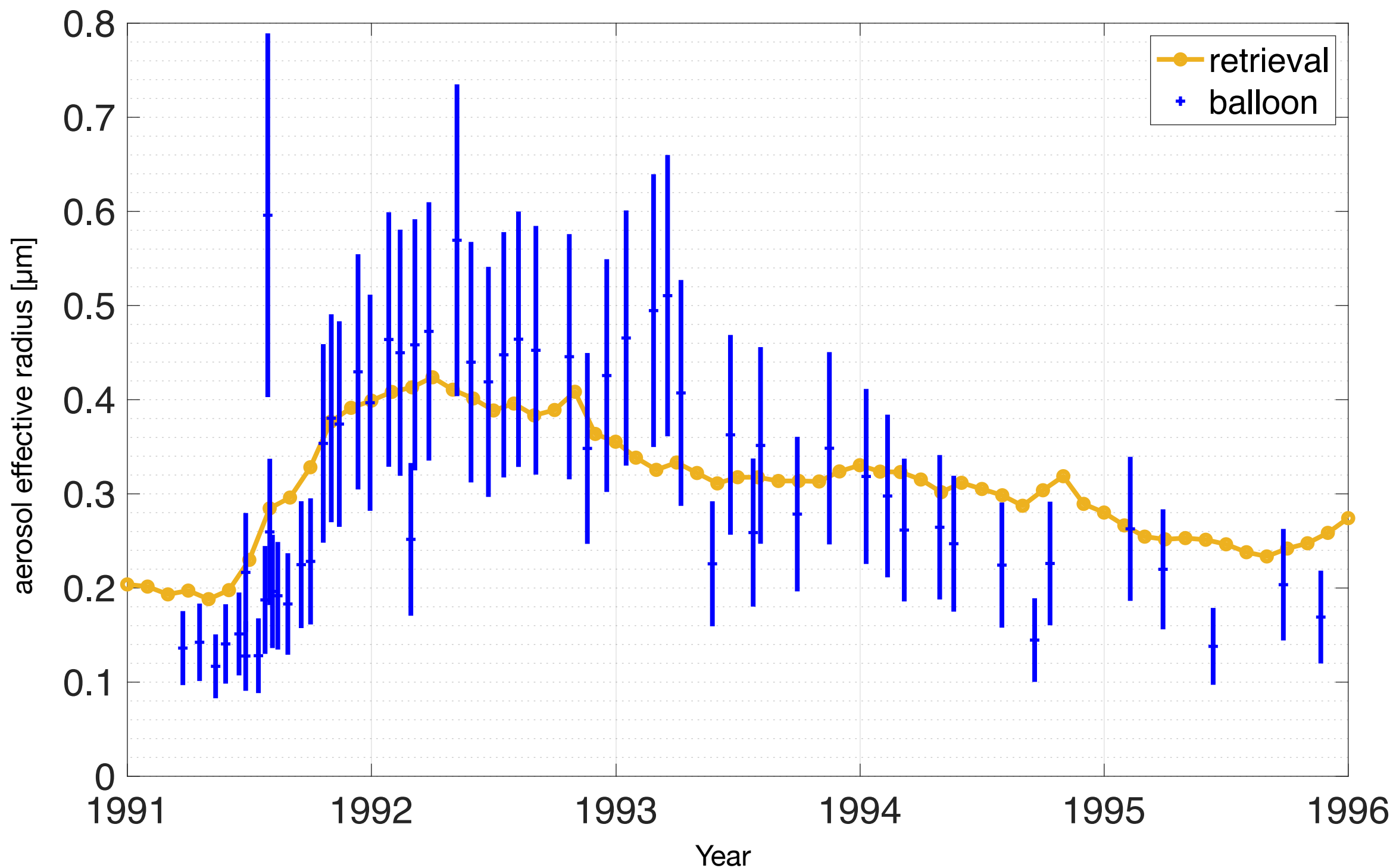
(a) Aerosol effective radius around Pinatubo
