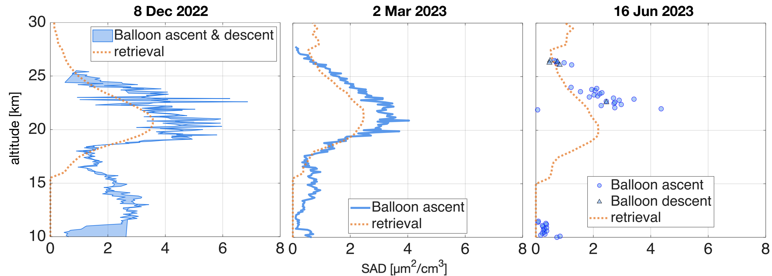
(b) Aerosol SAD after Hunga Tonga
