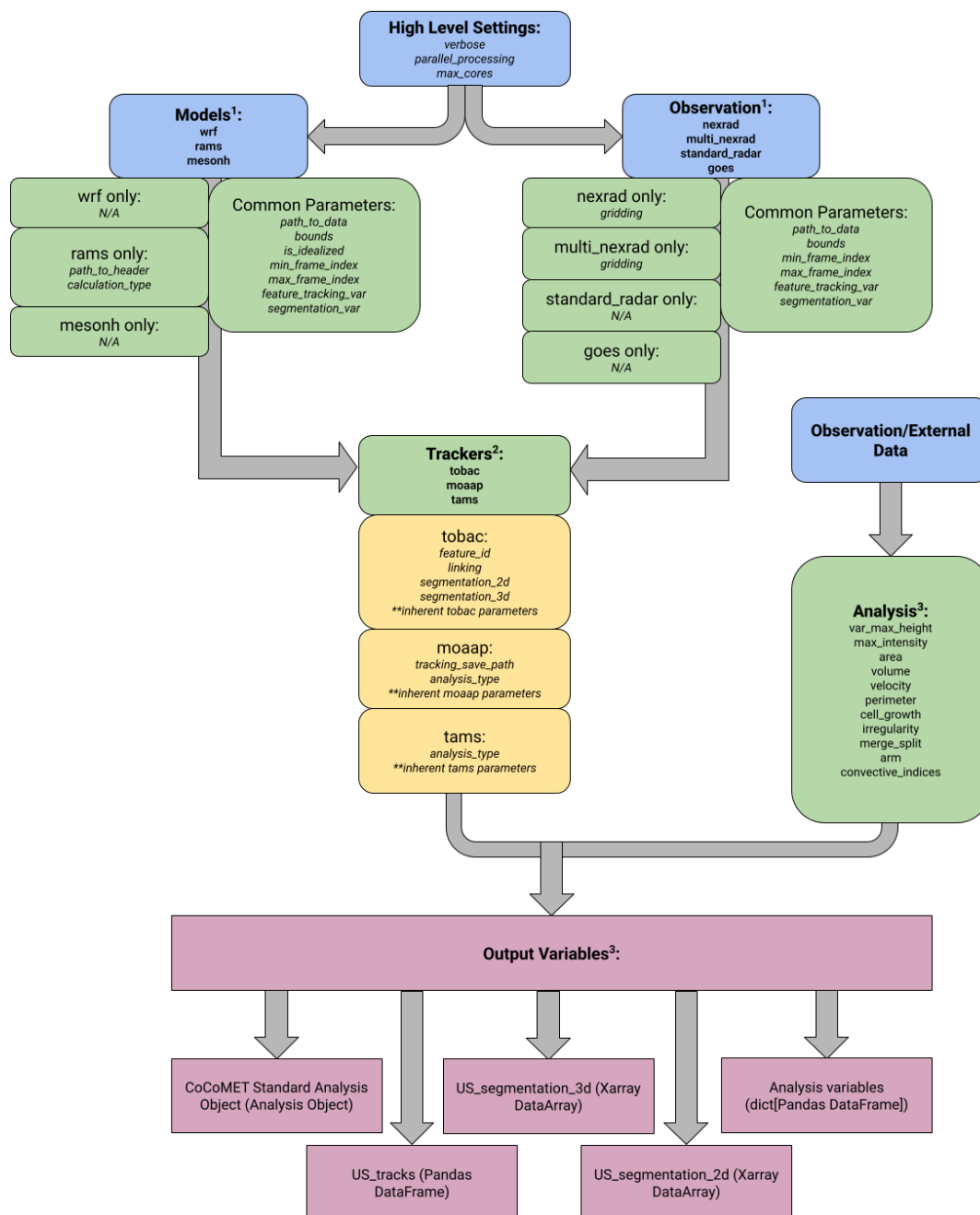
Figure 2. CoCoMET workflow highlighting the different input parameters for the configuration file, input data, and tracker options. Boxes marked as 1 are discussed in Sect. 2.1, as 2 are discussed in Sect. 2.2, and as 3 are discussed in Sect. 2.3.
