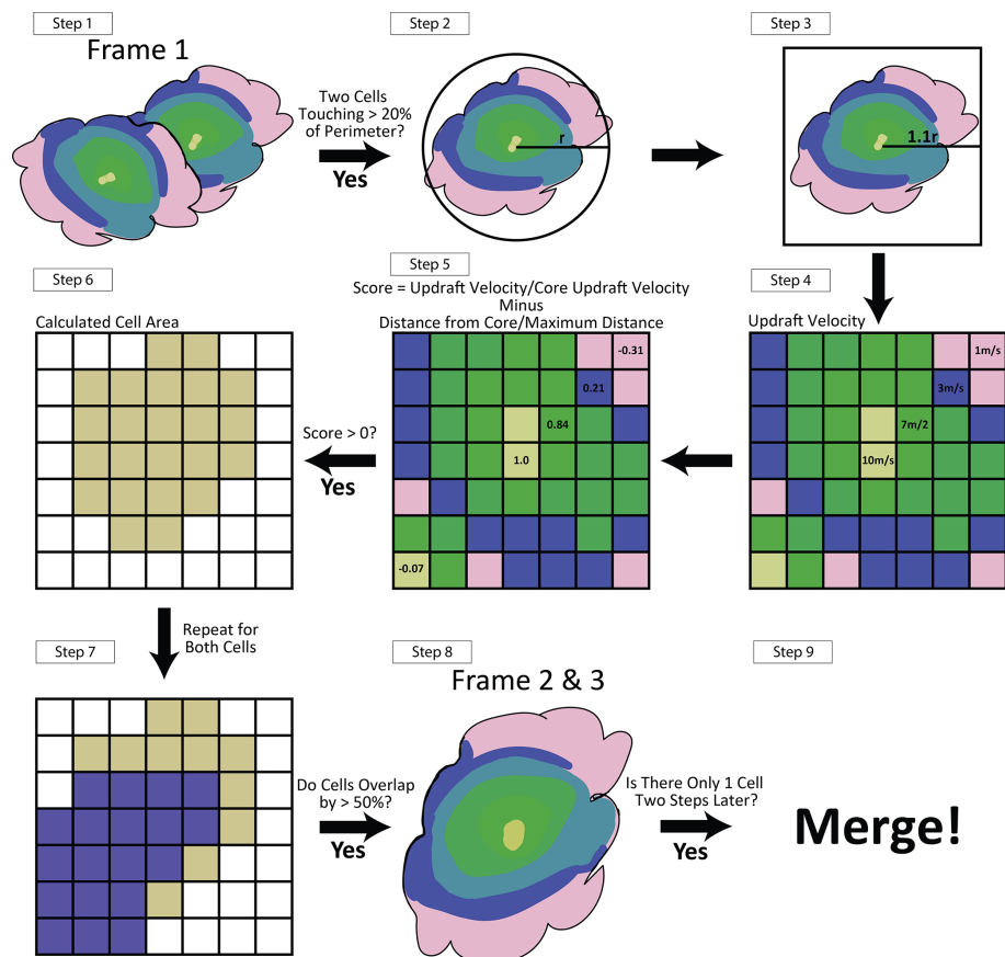
Figure 4. Illustration of steps for identifying mergers. An example input variable is updraft velocity at a certain height, using a threshold of 1 \text{ m s}^{-1} . Colors from green to purple represent the updraft velocity or score, ranging from high to low. The dust color in step 6 represents the calculated cell grids for cell 1 and purple for cells 2 in step 7.
