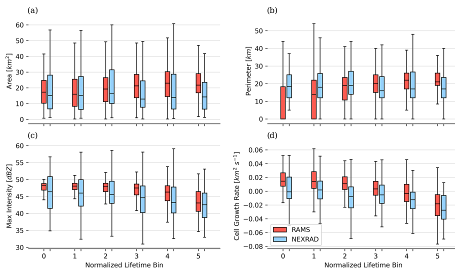
Figure 8. Box-whisker plot of tracked cell properties (both observed [NEXRAD] and simulated [RAMS]) as a function of the normalized lifetime bin. Only cells that last longer than 40 min and do not experience merging during their lifetime are included. 0 represents the first identification of the cell, and 5 indicates the termination of the tracked cell. Note that the unit of lifetime is in time units of minutes. The normalized lifetime is a unitless measurement.
