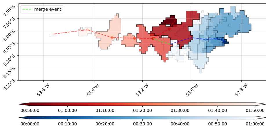
Figure 5. Example of a merging event detected by our new method using tracking outputs from tobac . The inputs for tobac are WRF simulations (Prein et al., 2022) of 2 km radar reflectivity at 1 km grid spacing for a deep convective case that occurred on 1 April 2014, in the Amazon. The tracking thresholds are 30, 40, and 50 dBZ. The cell in blue merges into the red one as both cells propagate toward the west.
