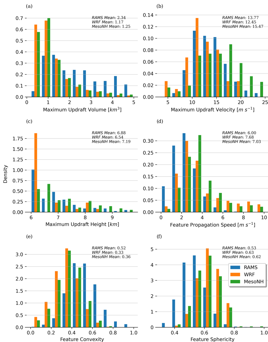
Figure 7. Histograms of tracked updraft properties using tobac based on simulations from WRF, Meso-HN, and RAMS for cases occurred on 19 June 2013 over the Houston region. Panels (b) and (c) are plotted only for updraft cells that extend higher than 6 km to highlight those deeper cores.
