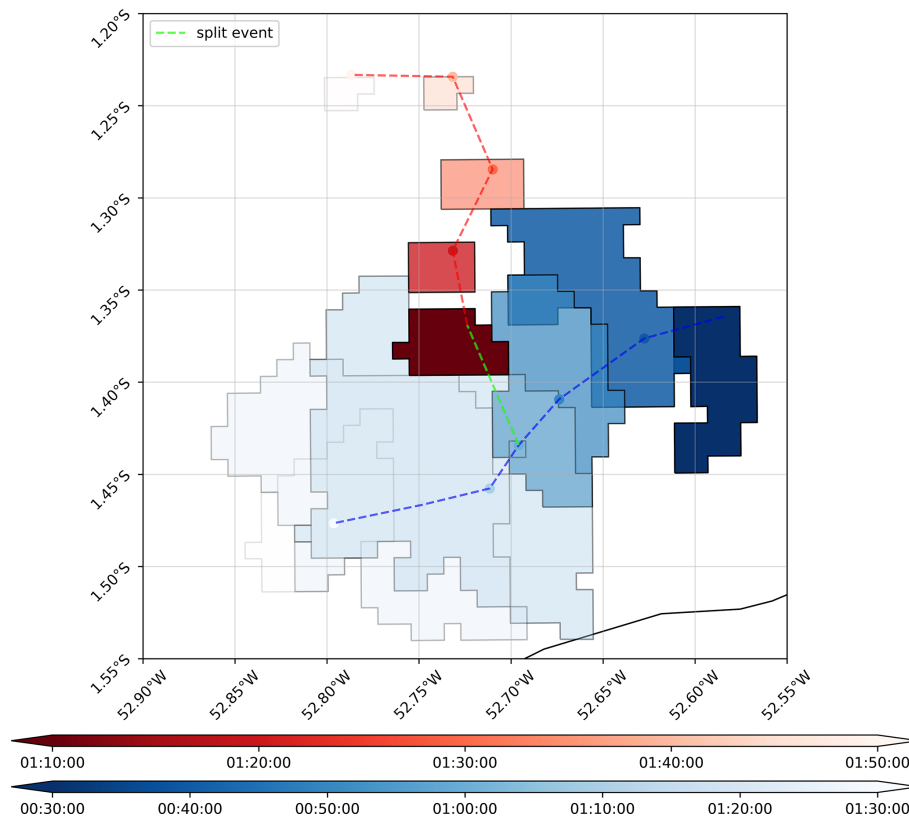
Figure 6. Example of a splitting event detected by our new method using tracking outputs from tobac . The inputs for tobac are WRF simulations (Prein et al., 2022) of 2 km radar reflectivity at 1 km grid spacing for a deep convective case that occurred on 1 April 2014, in the Amazon. The tracking thresholds are 30, 40, and 50 dBZ. The cell in blue splits into the blue and red cells.
