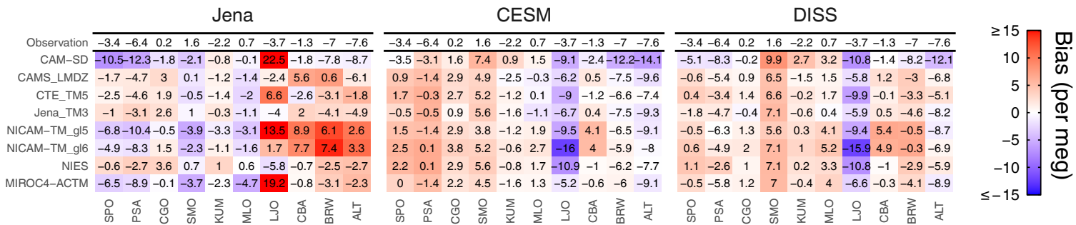
(b) APO Seasonal Cycle Amplitude (per meg)
