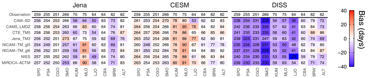
(c) APO Seasonal Minimum Day
