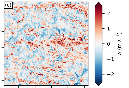
Resolved, \Delta_i = 2 m
