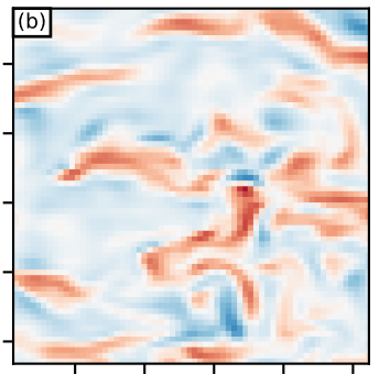
Resolved, \Delta_i = 16 m
