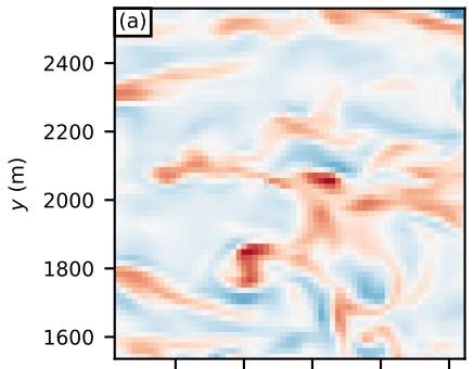
SLUrb, \Delta_i = 16 m
