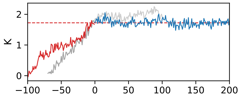
CNRM-ESM2-1
