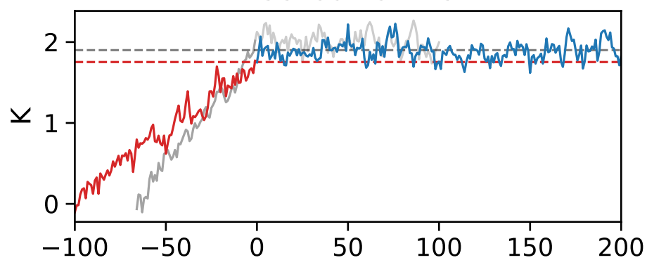
ACCESS-ESM1-5
