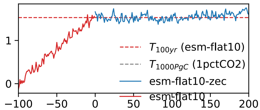
HadCM3LC-Bris
