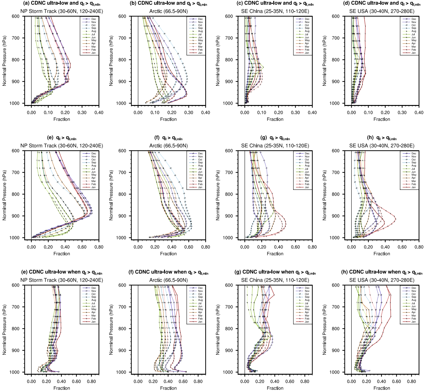
Figure S6. Monthly and regional mean vertical profiles of the joint probability P(\text{CDNC ultra-low} \cap \bar{q}_l \geq q_{l,\min}) (upper row), the probability P(\bar{q}_l \geq q_{l,\min}) (middle row), and the conditional probability P(\text{CDNC ultra-low} | \bar{q}_l \geq q_{l,\min}) (bottom row). The four columns correspond to different geographical regions, as indicated above the plot panels. All results shown in this figure correspond to q_{l,\min} = 10^{-15} \text{ g kg}^{-1} . The fractions (probabilities) were diagnosed from the free-running nc00 simulation (i.e., EAMv2 with no lower bound for CDNC) using output from the first simulation year after spin-up.
