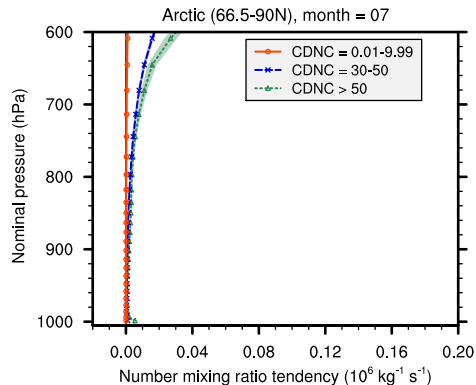
(b) # tend. associated with cld. frc. increase
