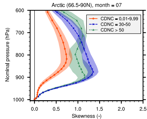
(g) Skewness of sub-grid w
