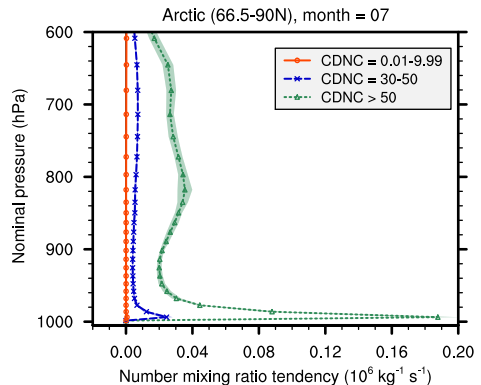
(a) # tend. due to cloud-base act.
