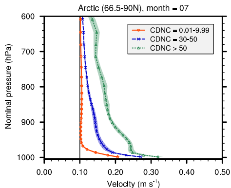
(e) w_{\text{act}}^* (assumed min. = 0.1)
