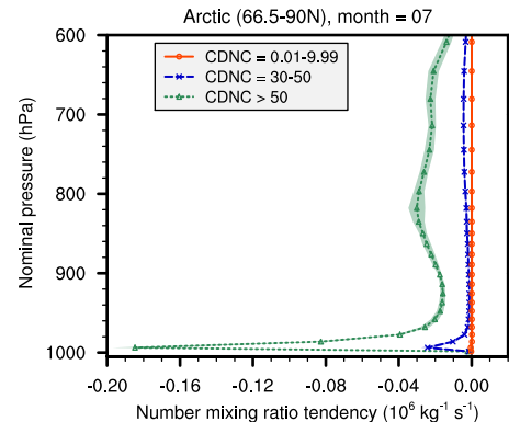
(c) # tend. due to turbulent mixing
