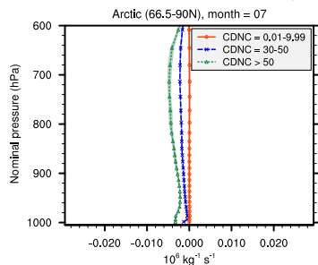
(b) Num. tend. due to resolved transport
