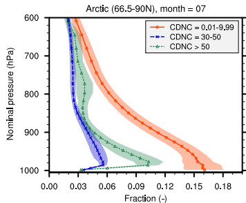
(a) Fractional freq. of occurrence
