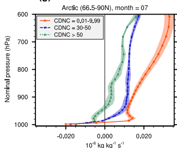
(g) Mass tend. due to CLUBB
