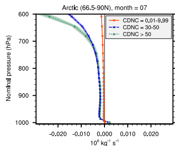
(d) Num. tend. due to cloud microphysics
