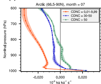
(h) Mass tend. due to cloud microphysics
