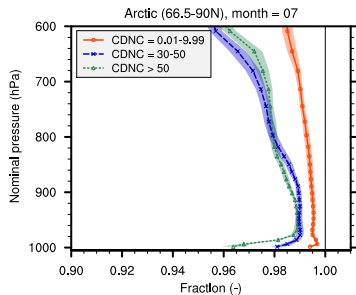
(e) Cloud fraction
