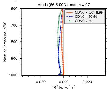
(f) Mass tend. due to resolved transport
