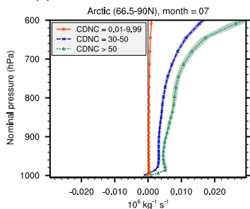
(c) Num. tend. due to DROPMIXNUC
