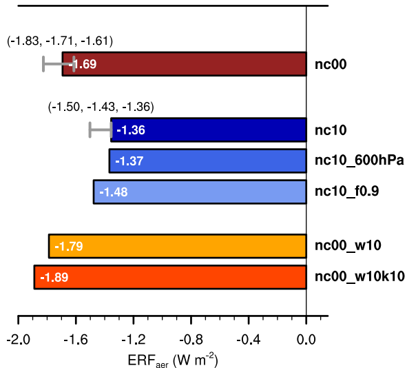
(a) Global annual mean \text{ERF}_{\text{aer}} ( \text{W m}^{-2} )
