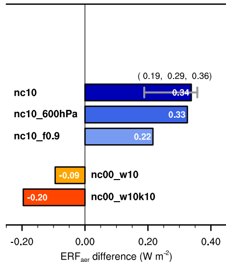
(b) Difference w.r.t. nc00 ( \text{W m}^{-2} )
