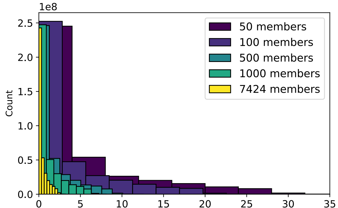
(b) Width of Extreme Temperature Probability Confidence Interval (%)
