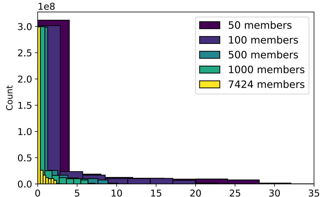
(a) Width of Extreme Temperature Probability Confidence Interval (%)
