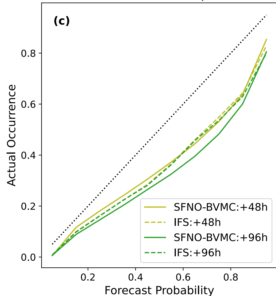
Reliability Diagram: 5th Percentile 2m Temperature
