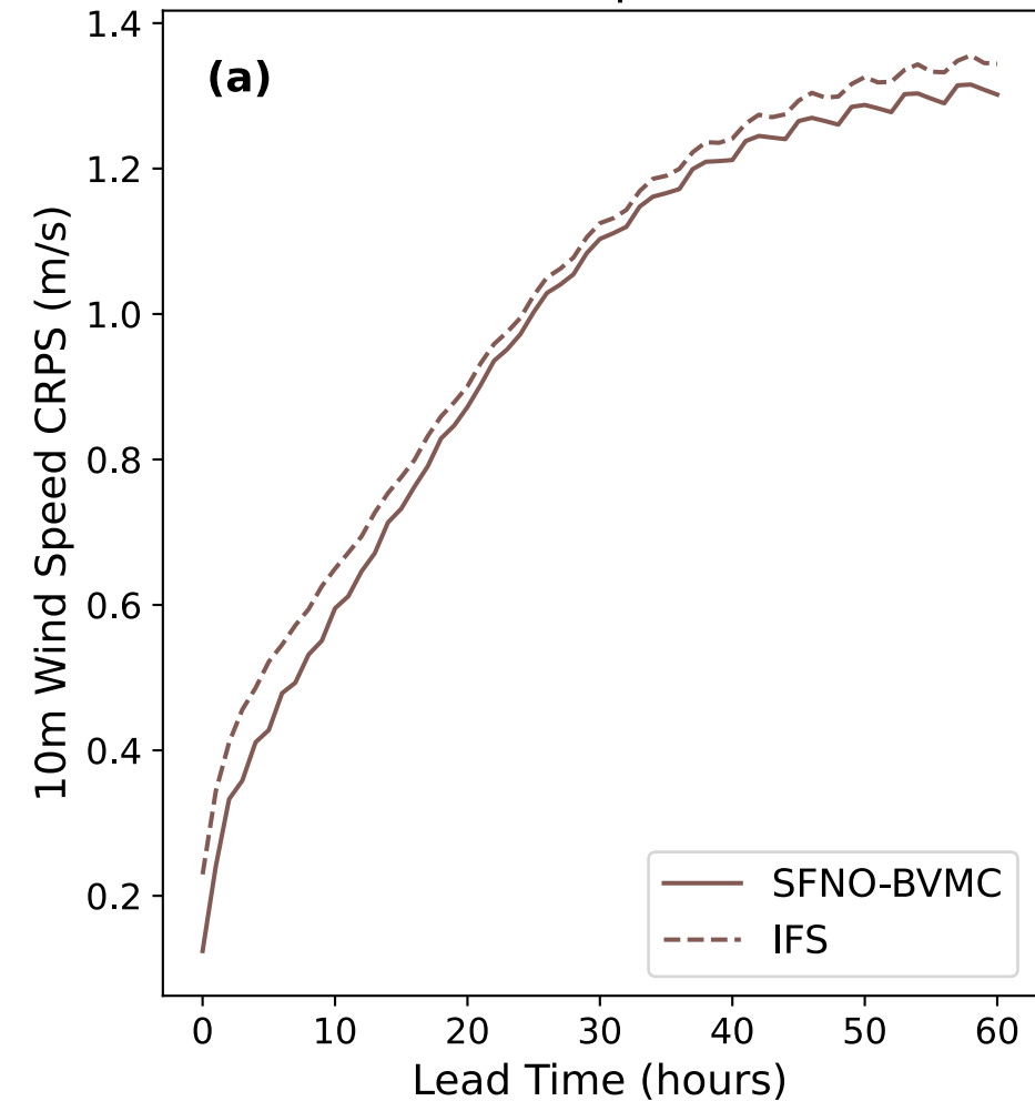
10m Wind Speed CRPS
