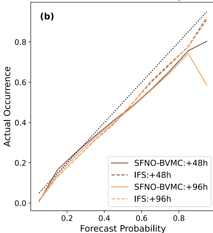
Reliability Diagram: 95th Percentile 10m Wind Speed
