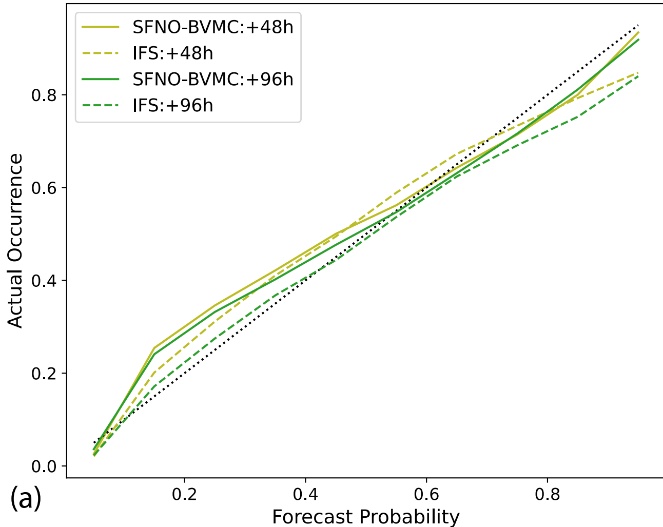
Heat Index Reliability Diagram (+48h, +96h Lead Time)
