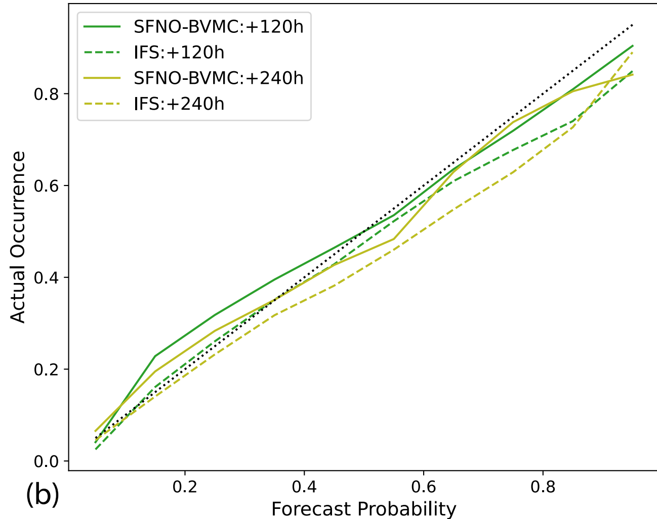
Heat Index Reliability Diagram (+120h, +240h Lead Time)
