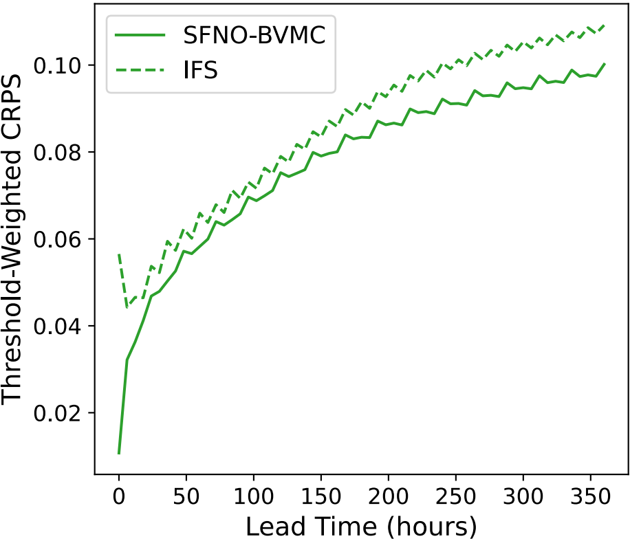
(c) 95th Percentile 2m Temperature Threshold-weighted CRPS
