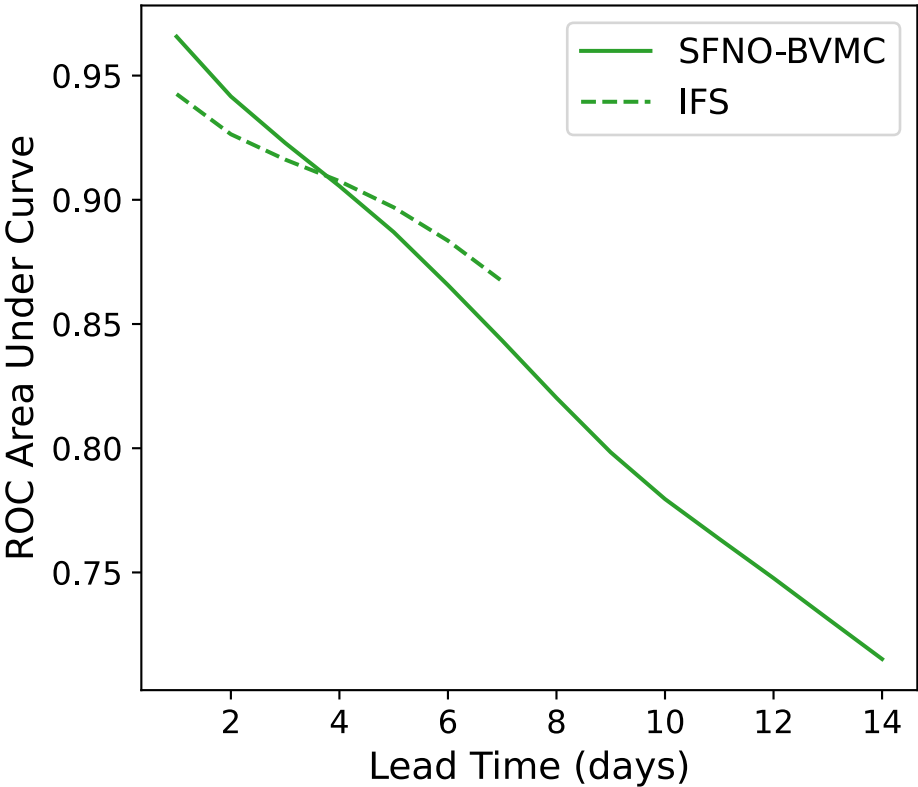
(b) 95th Percentile 2m Temperature Extreme Forecast Index ROC Curve
