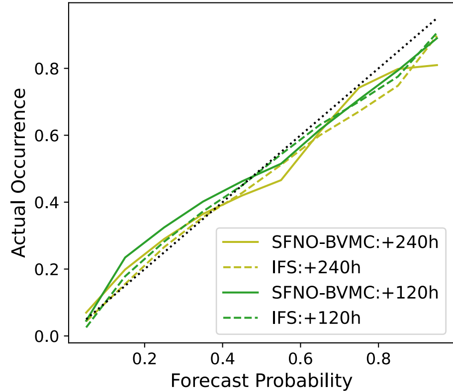
(a) 95th Percentile 2m Temperature Reliability Diagram
