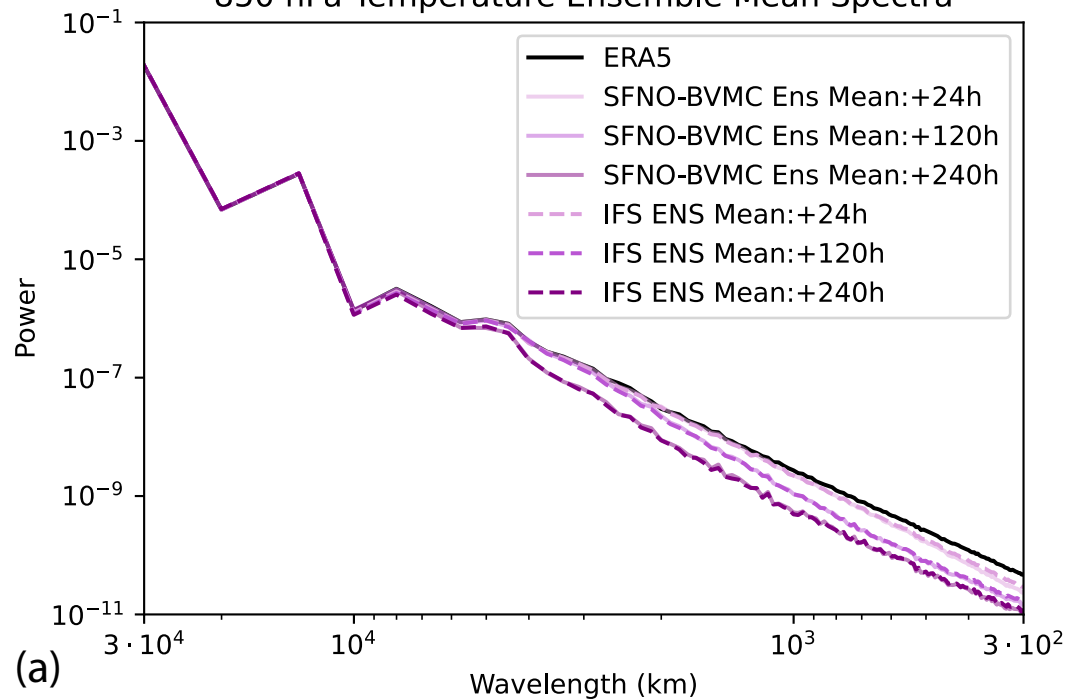
850 hPa Temperature Ensemble Mean Spectra
