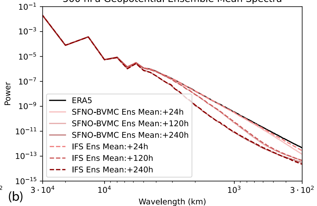
500 hPa Geopotential Ensemble Mean Spectra
