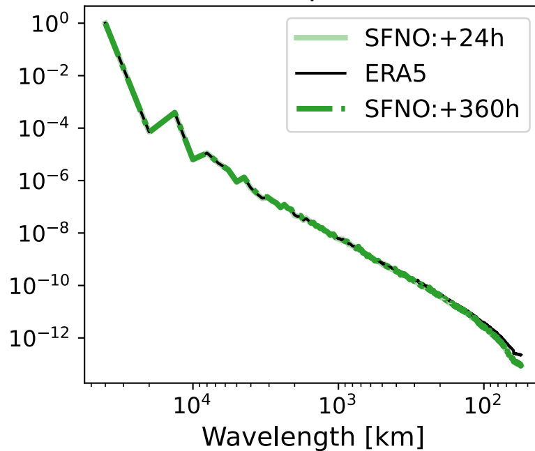
2m Temperature
