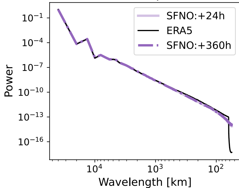
850hPa Temperature
