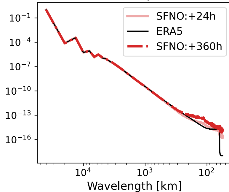
500 hPa Geopotential
