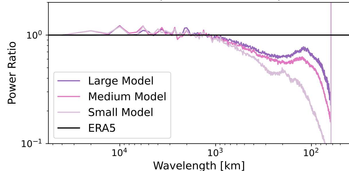
(b) 850 hPa Temperature Relative Spectra
