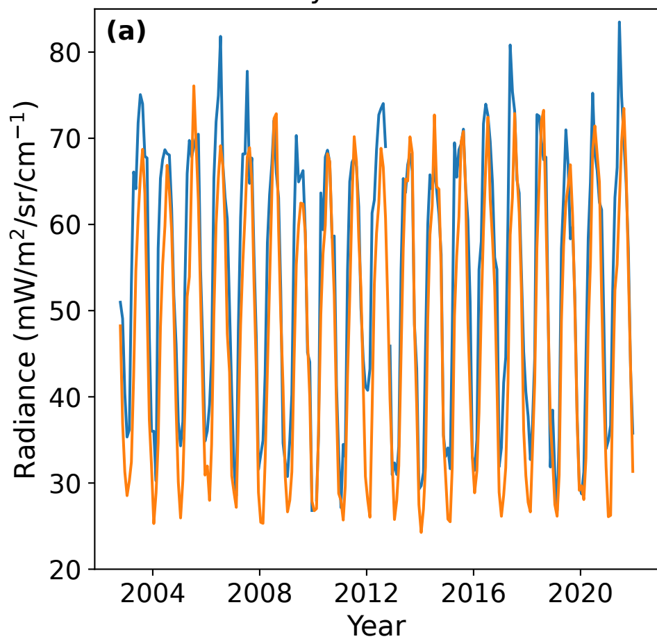
Daytime Orbits
