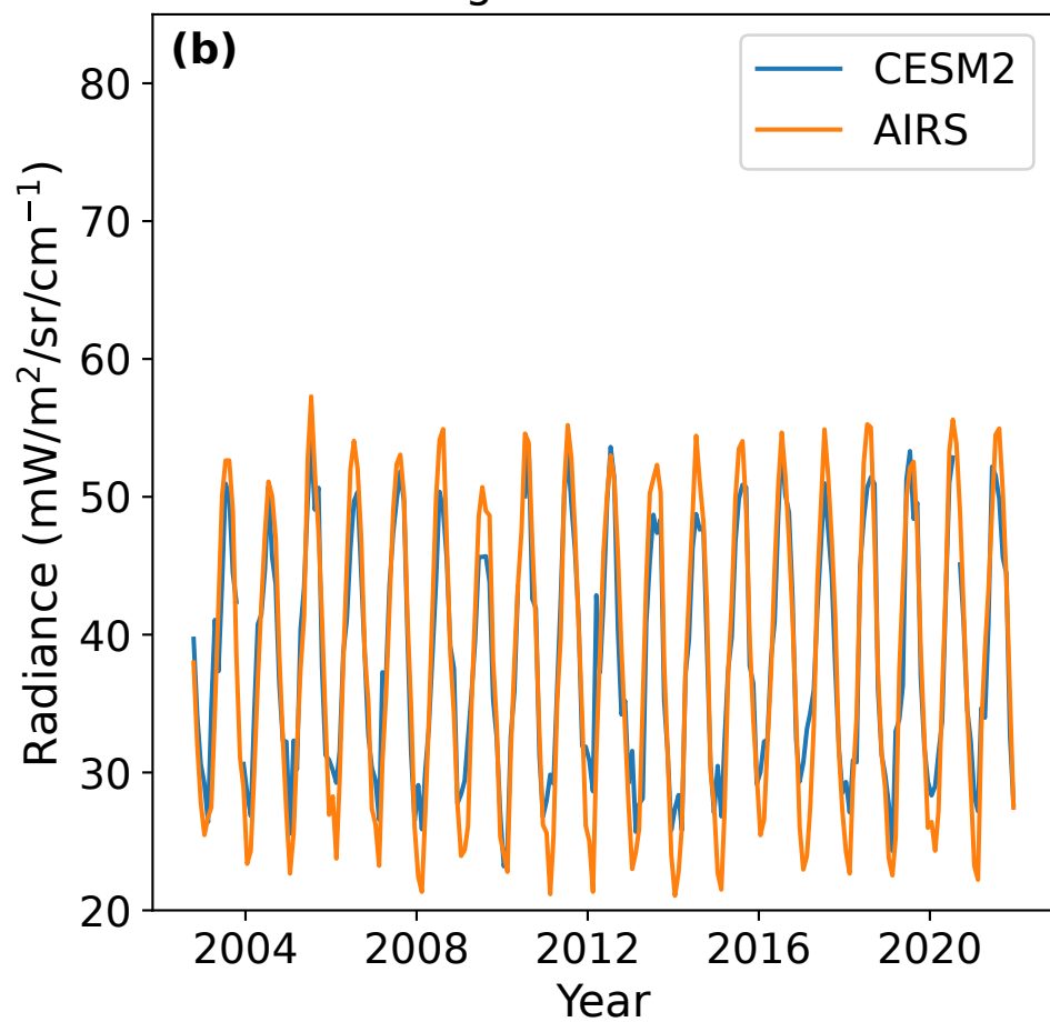
Nighttime Orbits
