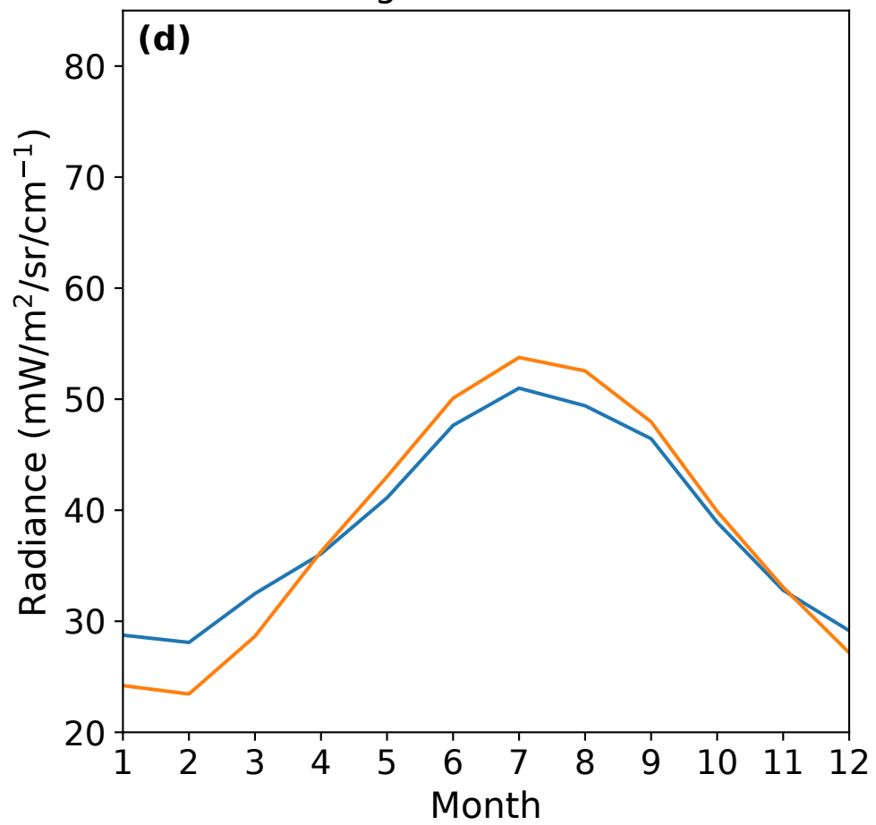
Nighttime Orbits
