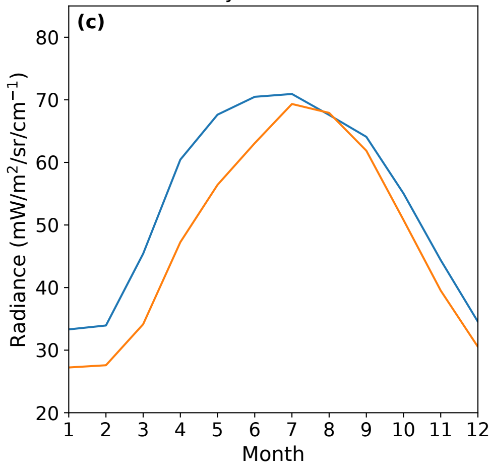
Daytime Orbits
