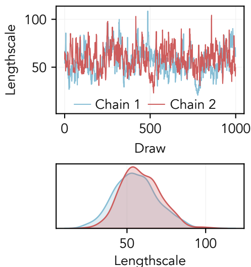
(b) Unimodal posterior: chains are stationary and mixed
