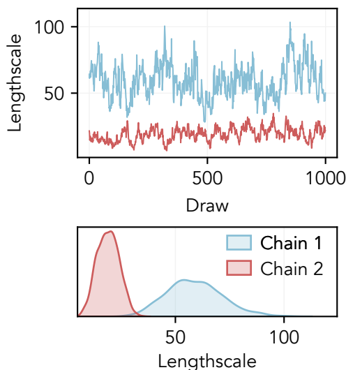
(a) Multimodal posterior: chains are stationary, but not mixed
