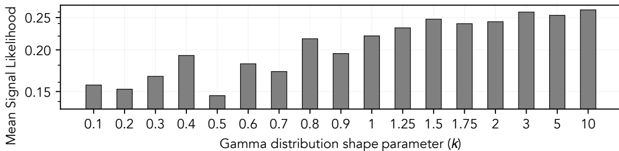
(c) MODEL PERFORMANCE FOR EPISODIC (LOW- k ) TO CONTINUOUS (HIGH- k ) DEPOSITION (4 SECTIONS)
