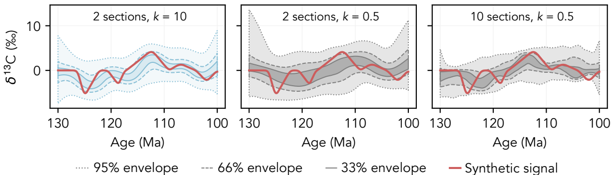
(a) OUTPUTS: INFERRED \delta^{13}\text{C} SIGNAL
