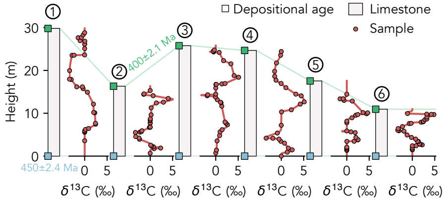
(b) TRANSLATING SIGNAL TO THE STRATIGRAPHIC RECORD
