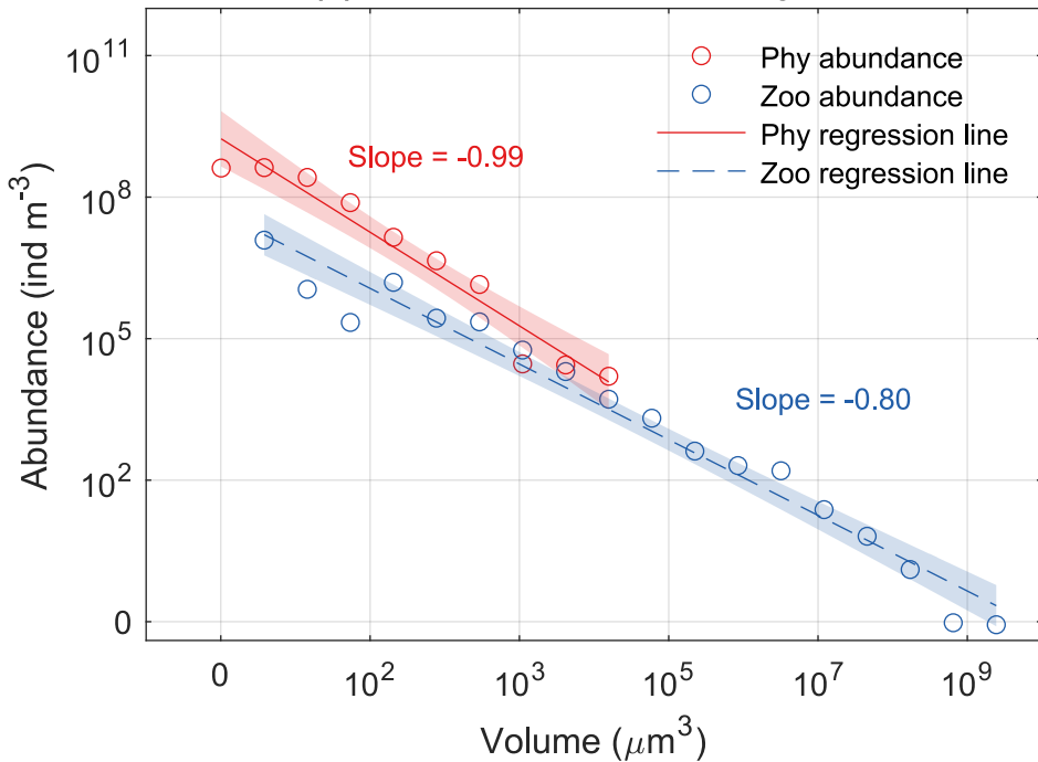
(a) Size Spectra for February 20 th
