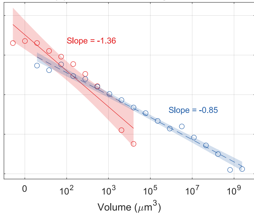
(b) Size Spectra for August 20 th
