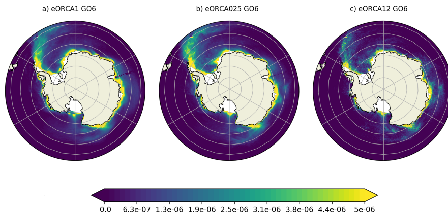
Figure S1. Annual mean of fresh water flux ( \text{kg.m}^{-2}.\text{s}^{-1} ) from iceberg melt calculated from GO6 integrations.
