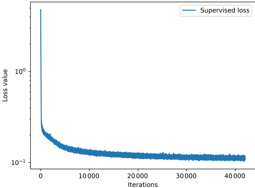
Training loss(es)
