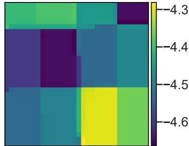
v wind [ \text{m s}^{-1} ]
