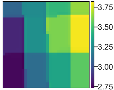
u wind [ \text{m s}^{-1} ]
