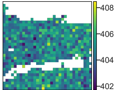
XCO2 [ppmv]
