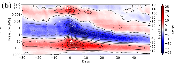
Deseasonalized anomalies
