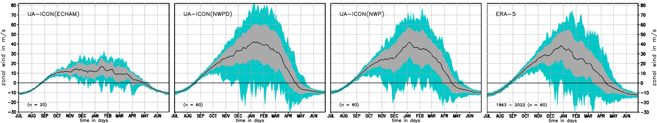
(b) Daily 10 hPa zonal mean zonal wind near 60^{\circ}\text{N}
