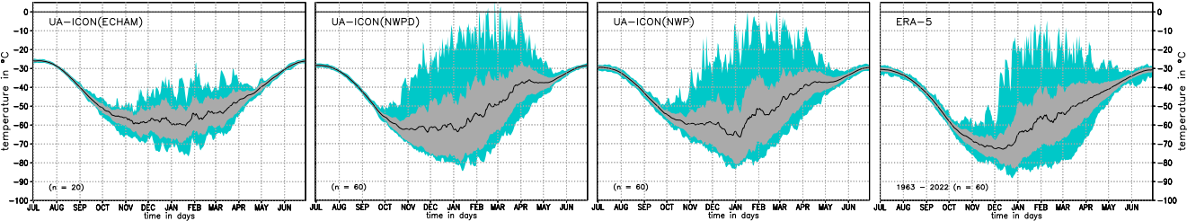
(a) Daily 10 hPa temperature near the North pole
